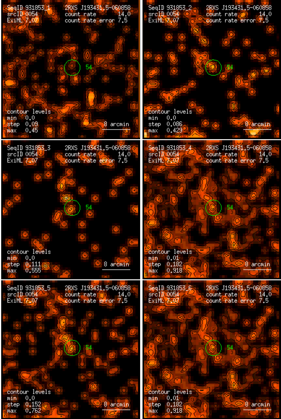
Figure 54: RASS 931853: detection 0054: band rate images, Gaussian filter: (1) PSPC channels 11 – 41, (2) 52 – 90, (3) 91 – 201, (4) 11 – 235, (5) 52 – 201, (6) 11 – 201. Broad band rates in counts/ks. Band rate contour levels in counts/ks/arcmin 2 .
