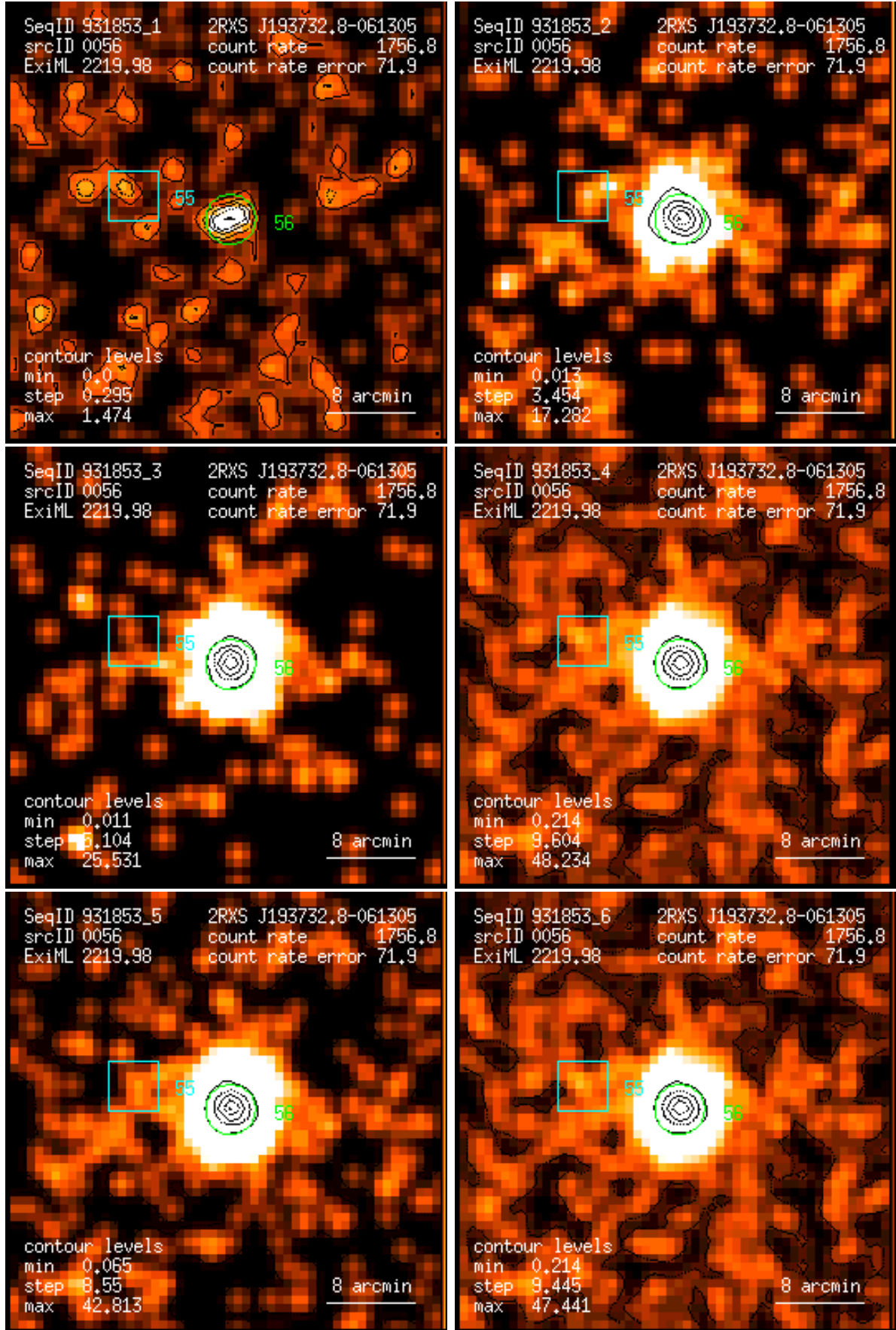
Figure 56: RASS 931853: detection 0056: band rate images, Gaussian filter: (1) PSPC channels 11 – 41, (2) 52 – 90, (3) 91 – 201, (4) 11 – 235, (5) 52 – 201, (6) 11 – 201. Broad band rates in counts/ks. Band rate contour levels in counts/ks/arcmin 2 .
