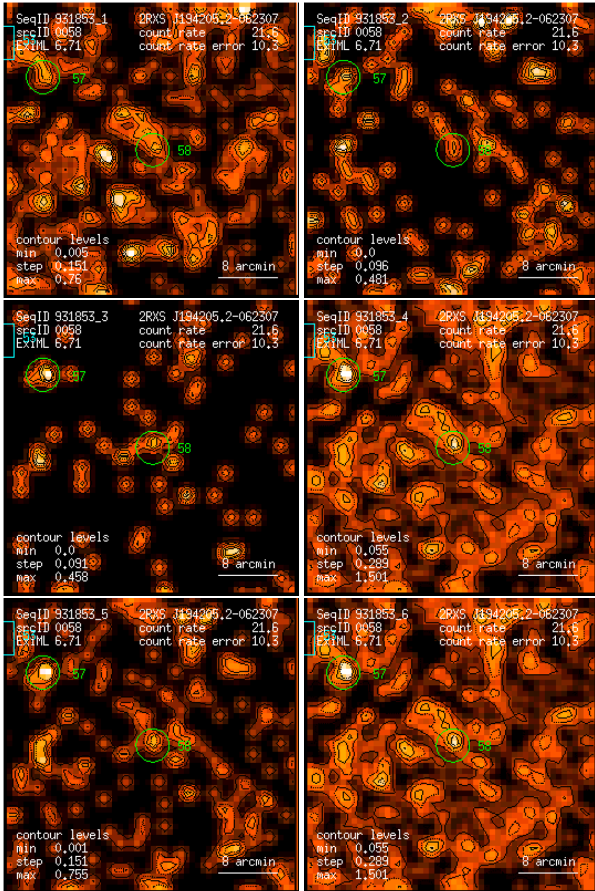
Figure 58: RASS 931853: detection 0058: band rate images, Gaussian filter: (1) PSPC channels 11 – 41, (2) 52 – 90, (3) 91 – 201, (4) 11 – 235, (5) 52 – 201, (6) 11 – 201. Broad band rates in counts/ks. Band rate contour levels in counts/ks/arcmin 2 .
