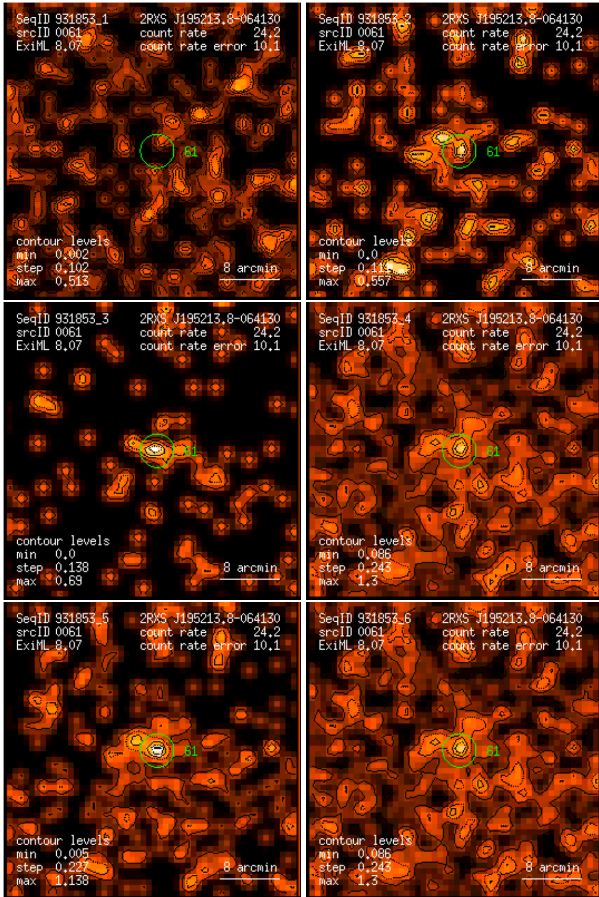
Figure 61: RASS 931853: detection 0061: band rate images, Gaussian filter: (1) PSPC channels 11 – 41, (2) 52 – 90, (3) 91 – 201, (4) 11 – 235, (5) 52 – 201, (6) 11 – 201. Broad band rates in counts/ks. Band rate contour levels in counts/ks/arcmin 2 .
