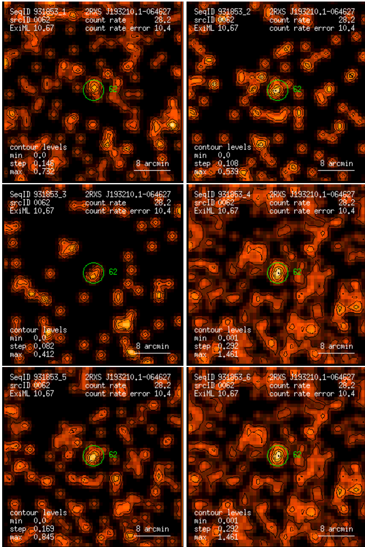
Figure 62: RASS 931853: detection 0062: band rate images, Gaussian filter: (1) PSPC channels 11 – 41, (2) 52 – 90, (3) 91 – 201, (4) 11 – 235, (5) 52 – 201, (6) 11 – 201. Broad band rates in counts/ks. Band rate contour levels in counts/ks/arcmin 2 .
