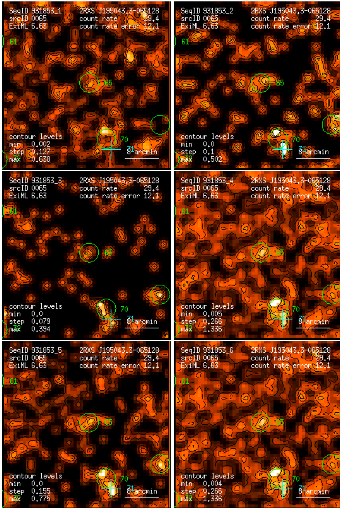
Figure 65: RASS 931853: detection 0065: band rate images, Gaussian filter: (1) PSPC channels 11 – 41, (2) 52 – 90, (3) 91 – 201, (4) 11 – 235, (5) 52 – 201, (6) 11 – 201. Broad band rates in counts/ks. Band rate contour levels in counts/ks/arcmin 2 .
