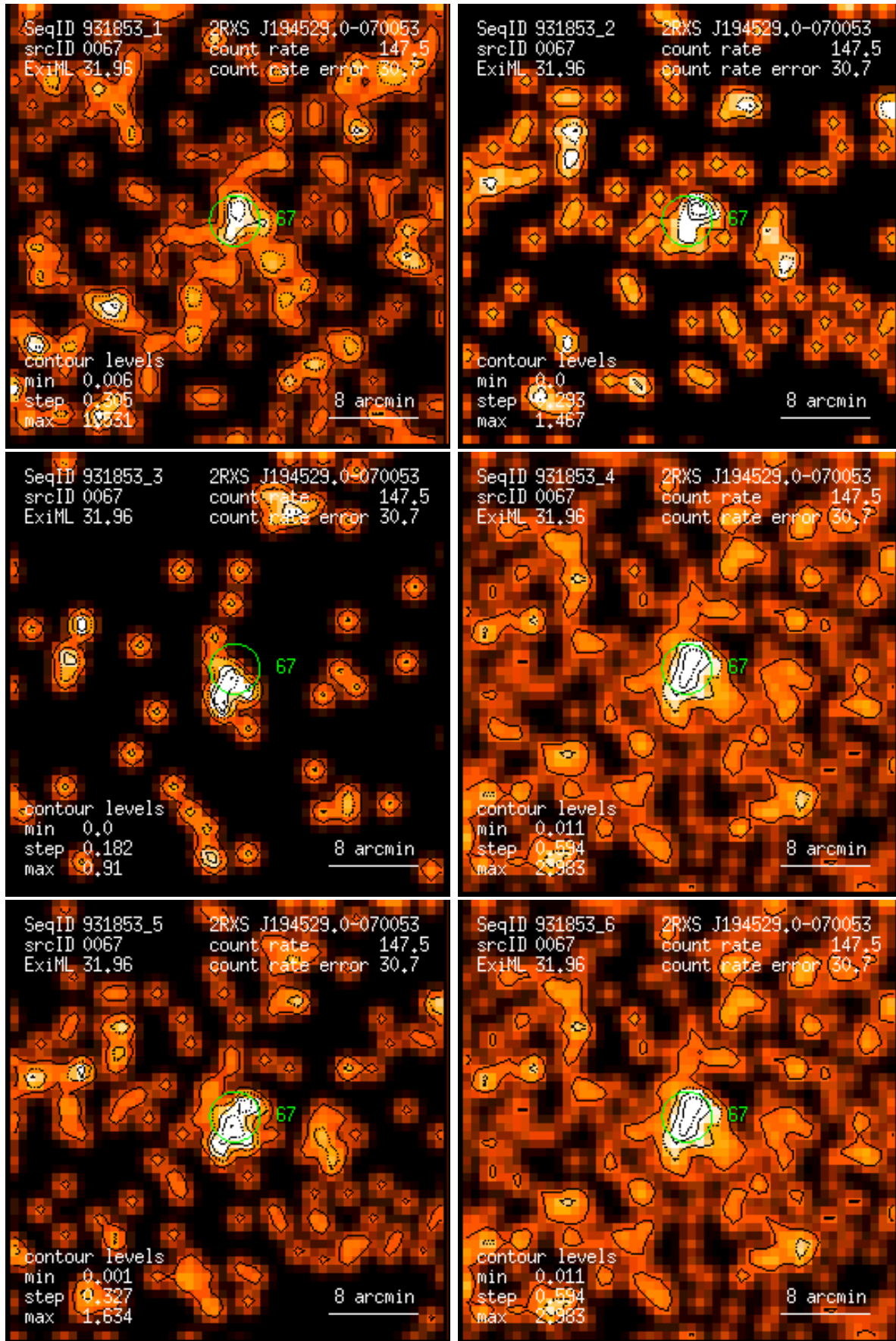
Figure 67: RASS 931853: detection 0067: band rate images, Gaussian filter: (1) PSPC channels 11 – 41, (2) 52 – 90, (3) 91 – 201, (4) 11 – 235, (5) 52 – 201, (6) 11 – 201. Broad band rates in counts/ks. Band rate contour levels in counts/ks/arcmin 2 .
