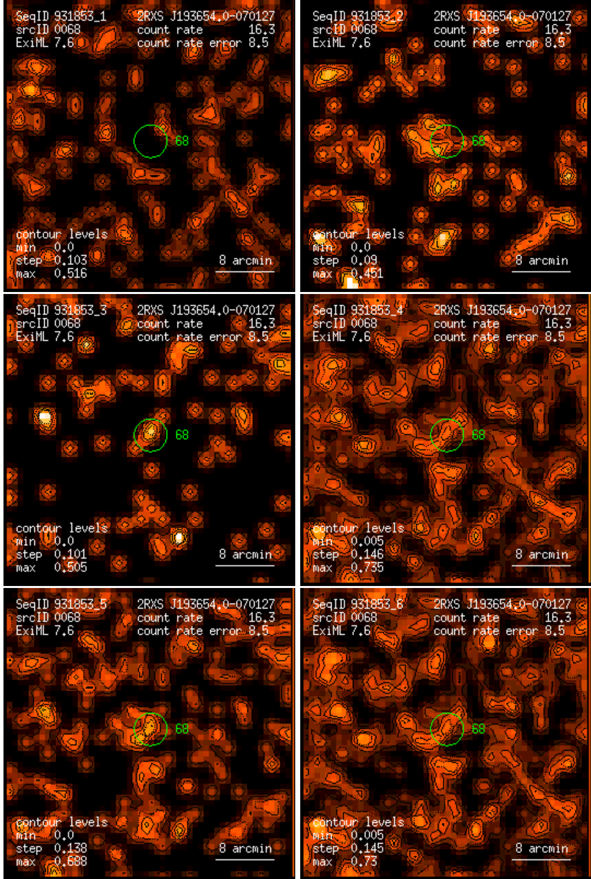
Figure 68: RASS 931853: detection 0068: band rate images, Gaussian filter: (1) PSPC channels 11 – 41, (2) 52 – 90, (3) 91 – 201, (4) 11 – 235, (5) 52 – 201, (6) 11 – 201. Broad band rates in counts/ks. Band rate contour levels in counts/ks/arcmin 2 .
