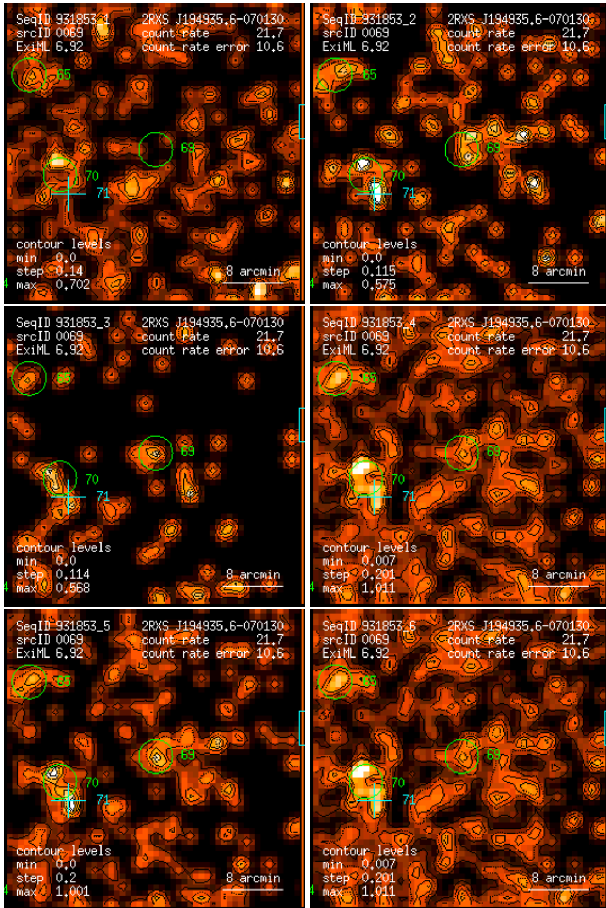
Figure 69: RASS 931853: detection 0069: band rate images, Gaussian filter: (1) PSPC channels 11 – 41, (2) 52 – 90, (3) 91 – 201, (4) 11 – 235, (5) 52 – 201, (6) 11 – 201. Broad band rates in counts/ks. Band rate contour levels in counts/ks/arcmin 2 .
