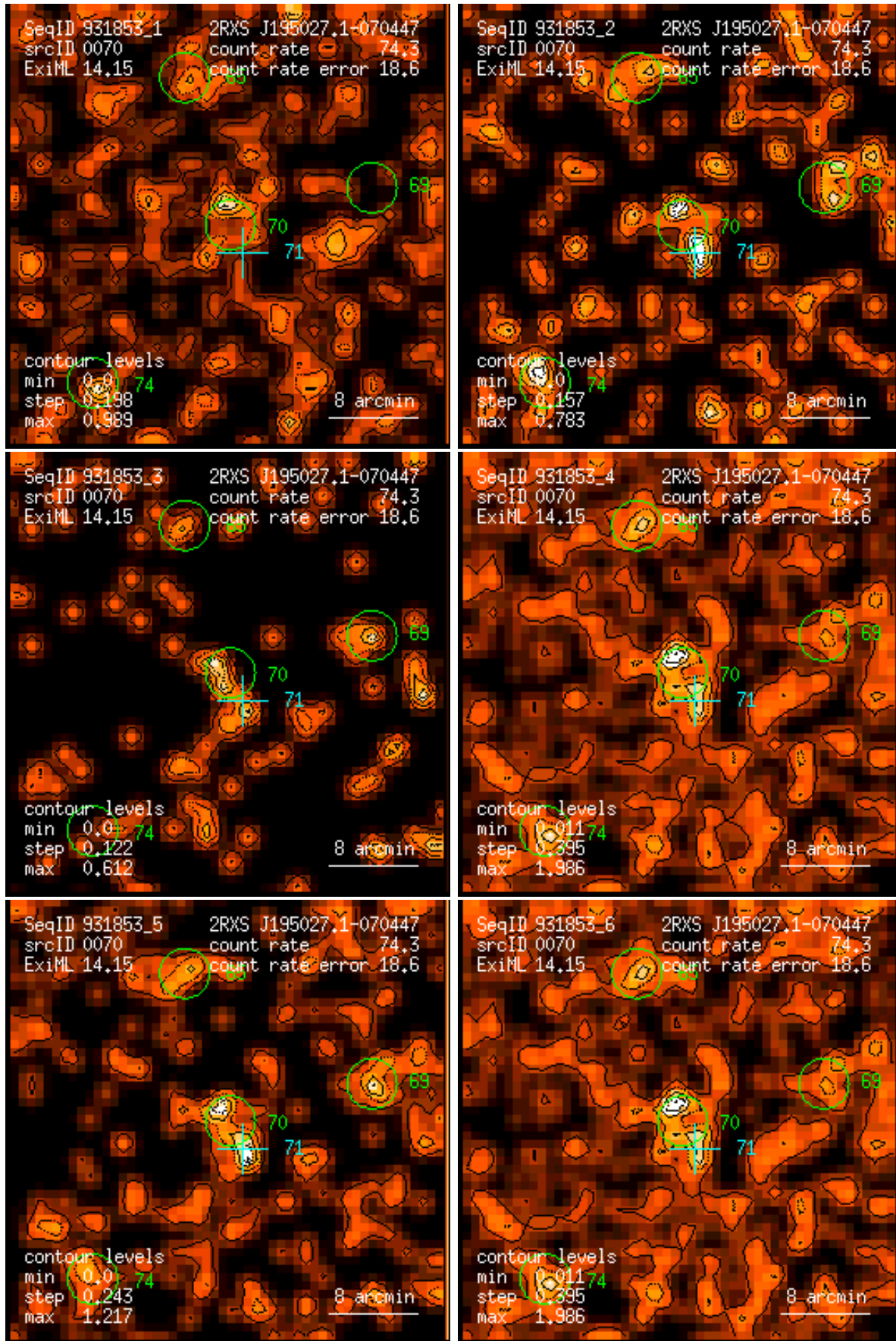
Figure 70: RASS 931853: detection 0070: band rate images, Gaussian filter: (1) PSPC channels 11 – 41, (2) 52 – 90, (3) 91 – 201, (4) 11 – 235, (5) 52 – 201, (6) 11 – 201. Broad band rates in counts/ks. Band rate contour levels in counts/ks/arcmin 2 .
