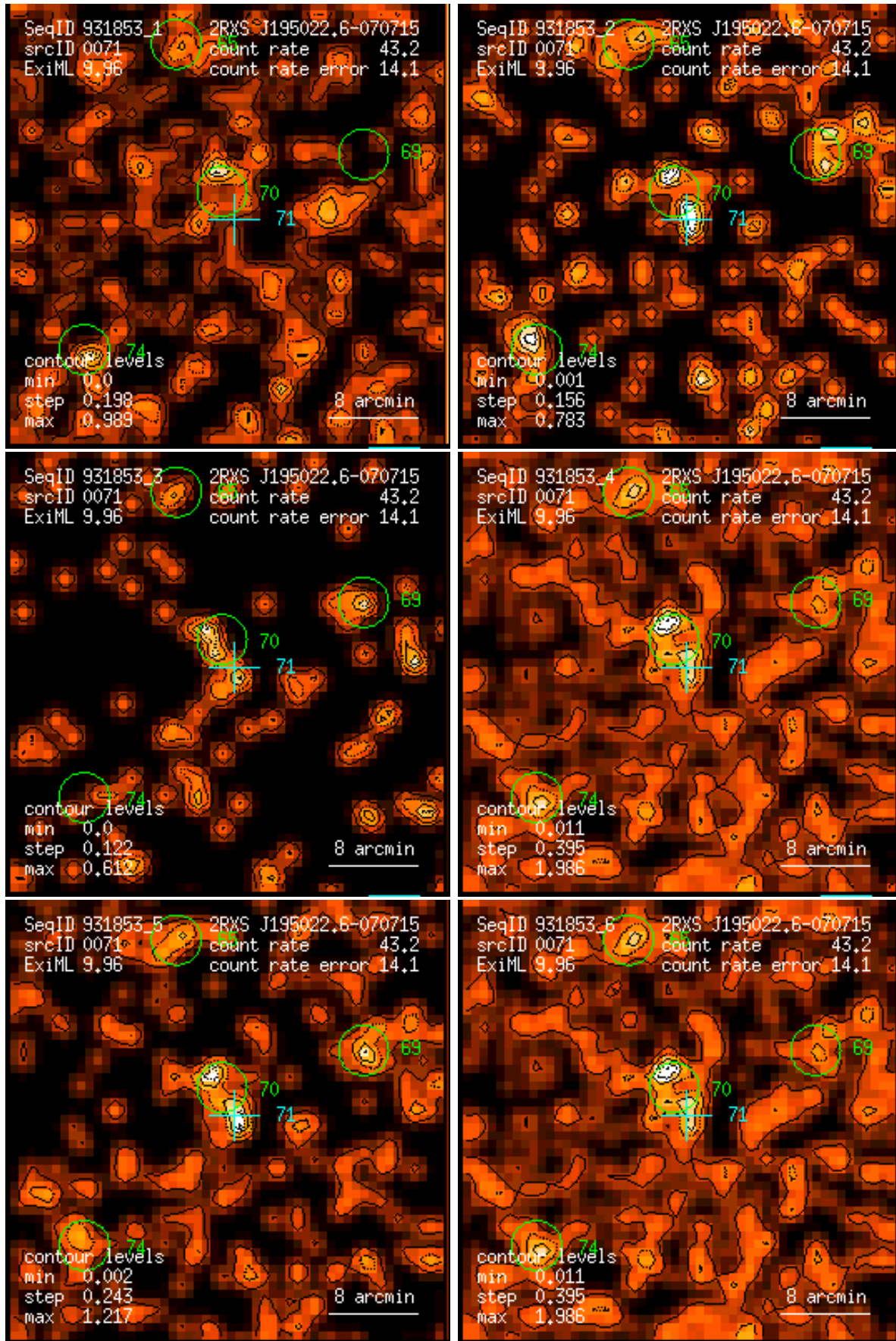
Figure 71: RASS 931853: detection 0071: band rate images, Gaussian filter: (1) PSPC channels 11 – 41, (2) 52 – 90, (3) 91 – 201, (4) 11 – 235, (5) 52 – 201, (6) 11 – 201. Broad band rates in counts/ks. Band rate contour levels in counts/ks/arcmin 2 .
