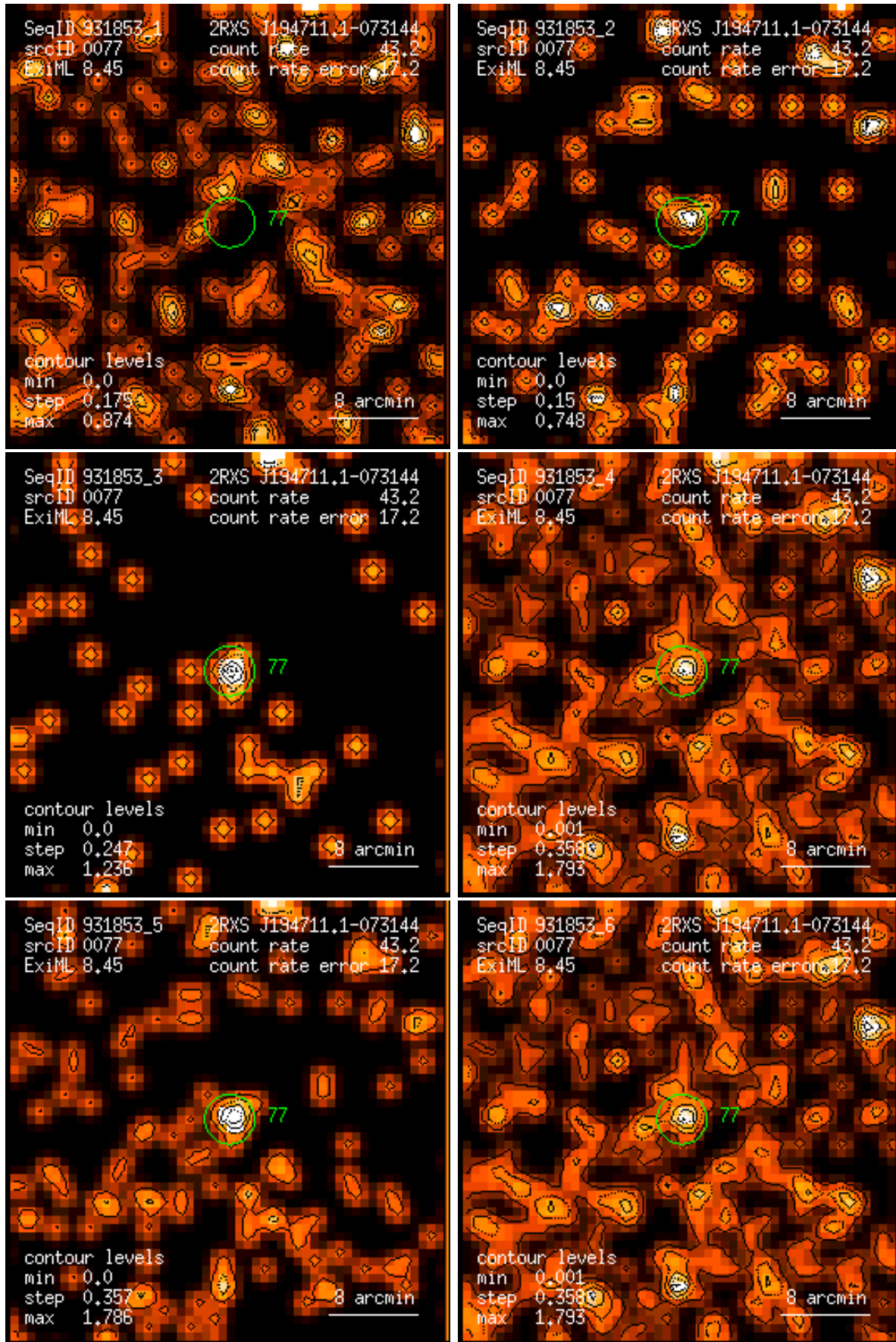
Figure 77: RASS 931853: detection 0077: band rate images, Gaussian filter: (1) PSPC channels 11 – 41, (2) 52 – 90, (3) 91 – 201, (4) 11 – 235, (5) 52 – 201, (6) 11 – 201. Broad band rates in counts/ks. Band rate contour levels in counts/ks/arcmin 2 .
