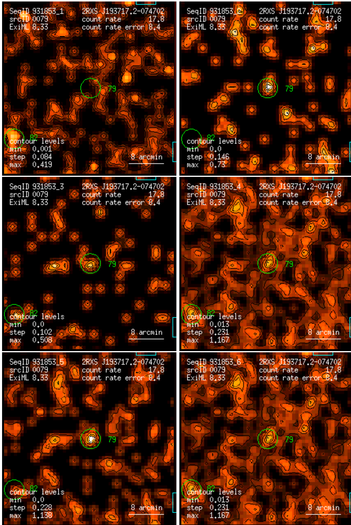
Figure 79: RASS 931853: detection 0079: band rate images, Gaussian filter: (1) PSPC channels 11 – 41, (2) 52 – 90, (3) 91 – 201, (4) 11 – 235, (5) 52 – 201, (6) 11 – 201. Broad band rates in counts/ks. Band rate contour levels in counts/ks/arcmin 2 .
