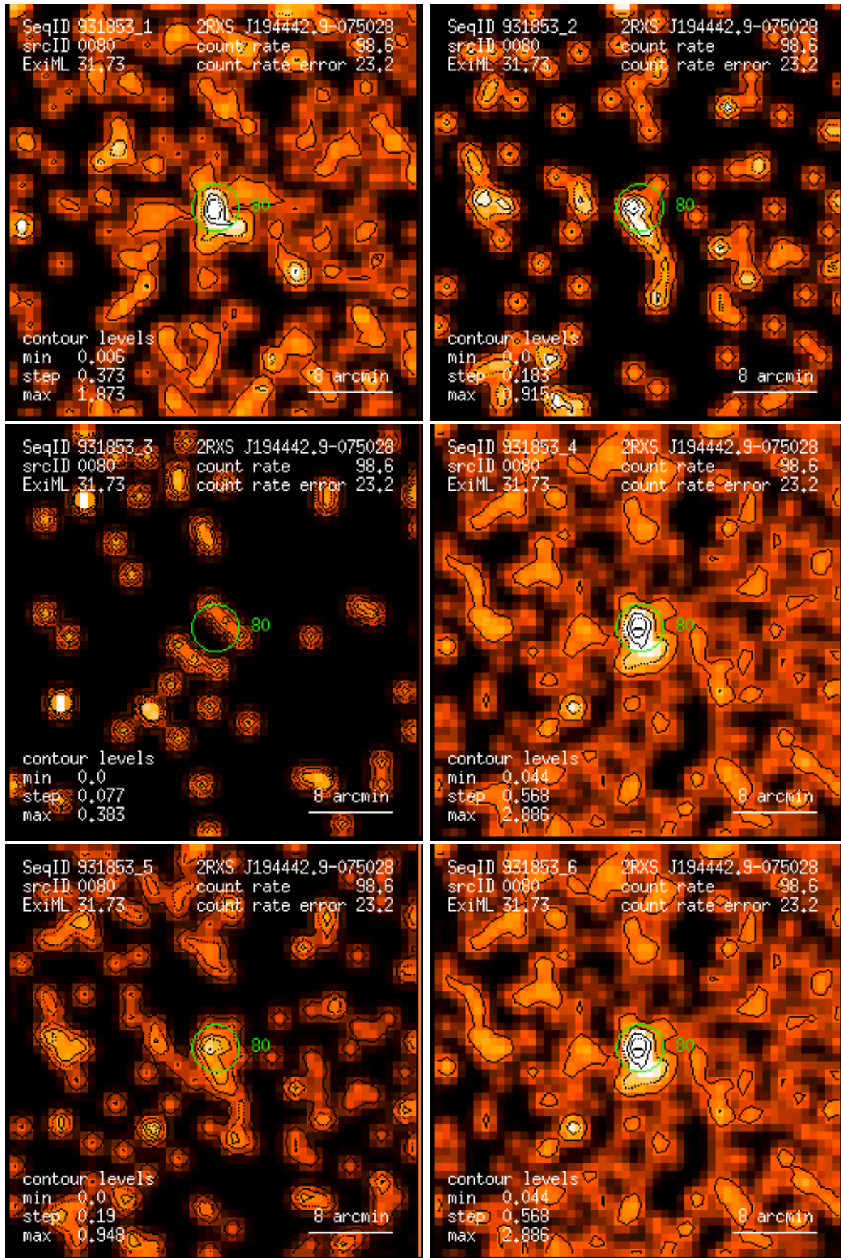
Figure 80: RASS 931853: detection 0080: band rate images, Gaussian filter: (1) PSPC channels 11 – 41, (2) 52 – 90, (3) 91 – 201, (4) 11 – 235, (5) 52 – 201, (6) 11 – 201. Broad band rates in counts/ks. Band rate contour levels in counts/ks/arcmin 2 .
