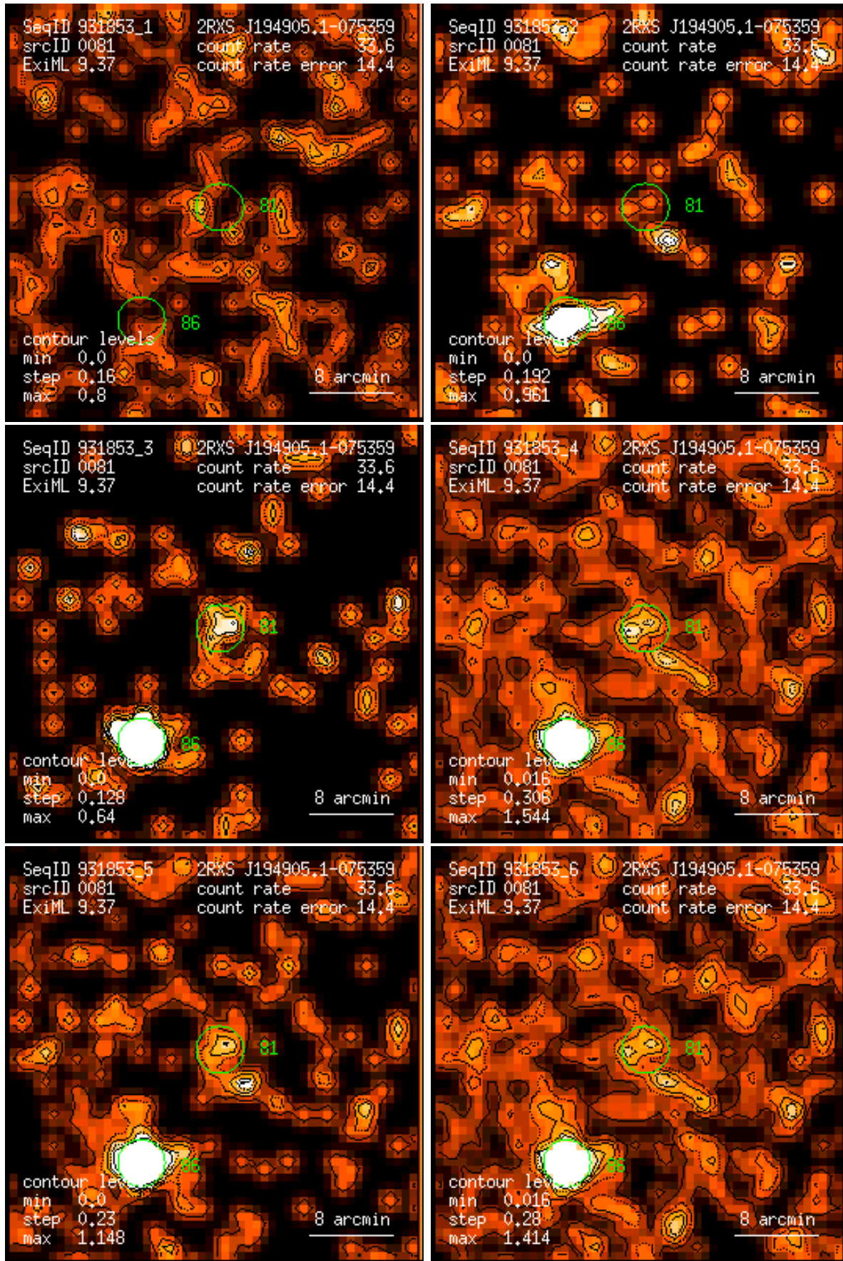
Figure 81: RASS 931853: detection 0081: band rate images, Gaussian filter: (1) PSPC channels 11 – 41, (2) 52 – 90, (3) 91 – 201, (4) 11 – 235, (5) 52 – 201, (6) 11 – 201. Broad band rates in counts/ks. Band rate contour levels in counts/ks/arcmin 2 .
