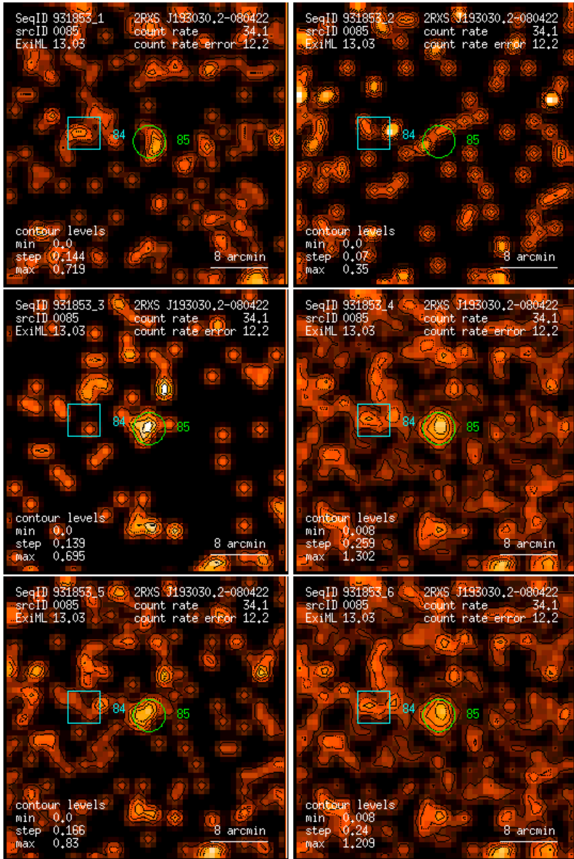
Figure 85: RASS 931853: detection 0085: band rate images, Gaussian filter: (1) PSPC channels 11 – 41, (2) 52 – 90, (3) 91 – 201, (4) 11 – 235, (5) 52 – 201, (6) 11 – 201. Broad band rates in counts/ks. Band rate contour levels in counts/ks/arcmin 2 .
