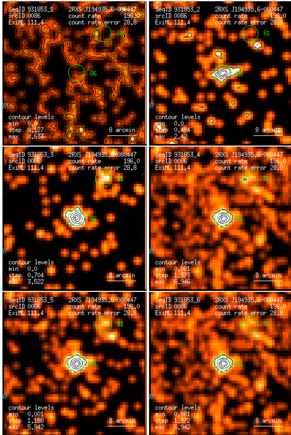
Figure 86: RASS 931853: detection 0086: band rate images, Gaussian filter: (1) PSPC channels 11 – 41, (2) 52 – 90, (3) 91 – 201, (4) 11 – 235, (5) 52 – 201, (6) 11 – 201. Broad band rates in counts/ks. Band rate contour levels in counts/ks/arcmin 2 .
