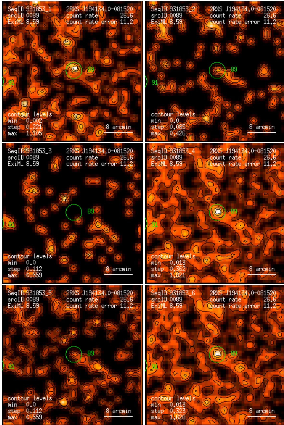
Figure 89: RASS 931853: detection 0089: band rate images, Gaussian filter: (1) PSPC channels 11 – 41, (2) 52 – 90, (3) 91 – 201, (4) 11 – 235, (5) 52 – 201, (6) 11 – 201. Broad band rates in counts/ks. Band rate contour levels in counts/ks/arcmin 2 .
