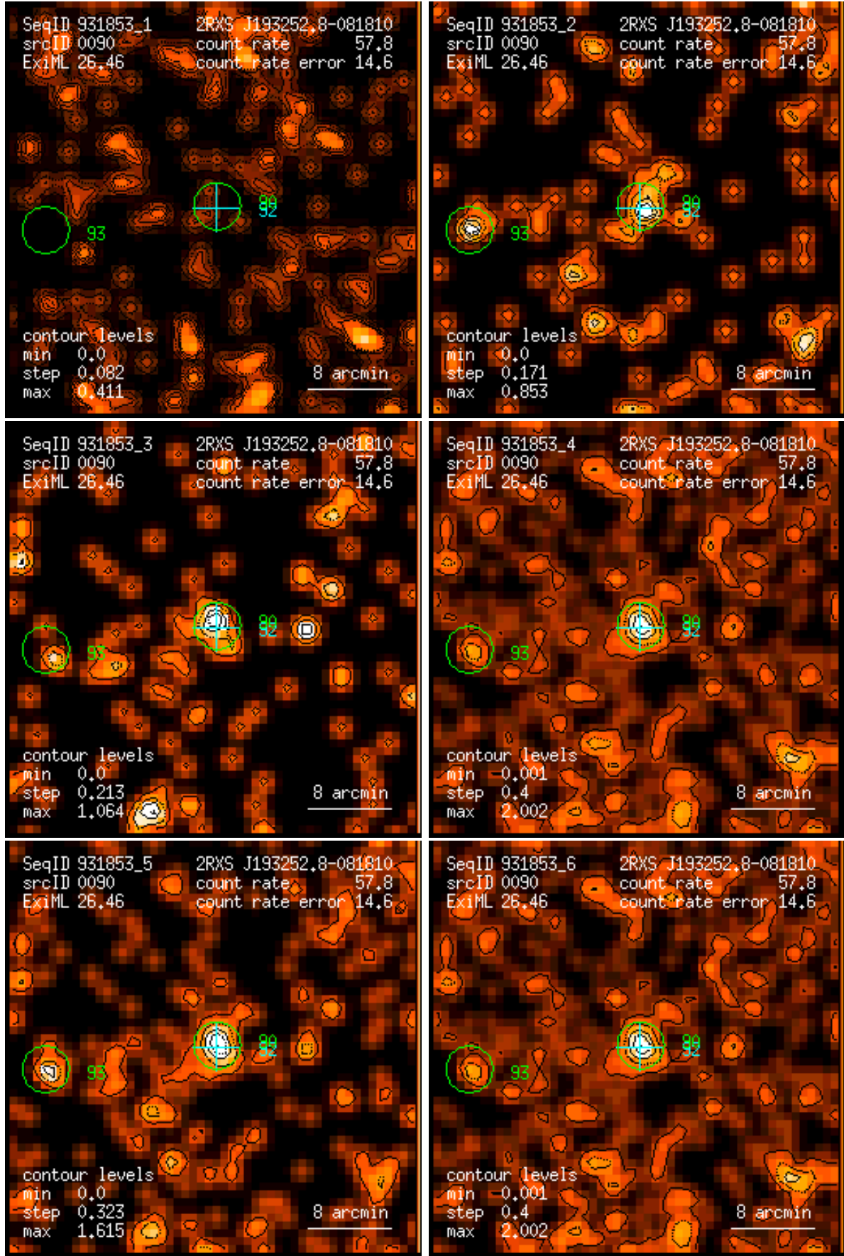
Figure 90: RASS 931853: detection 0090: band rate images, Gaussian filter: (1) PSPC channels 11 – 41, (2) 52 – 90, (3) 91 – 201, (4) 11 – 235, (5) 52 – 201, (6) 11 – 201. Broad band rates in counts/ks. Band rate contour levels in counts/ks/arcmin 2 .
