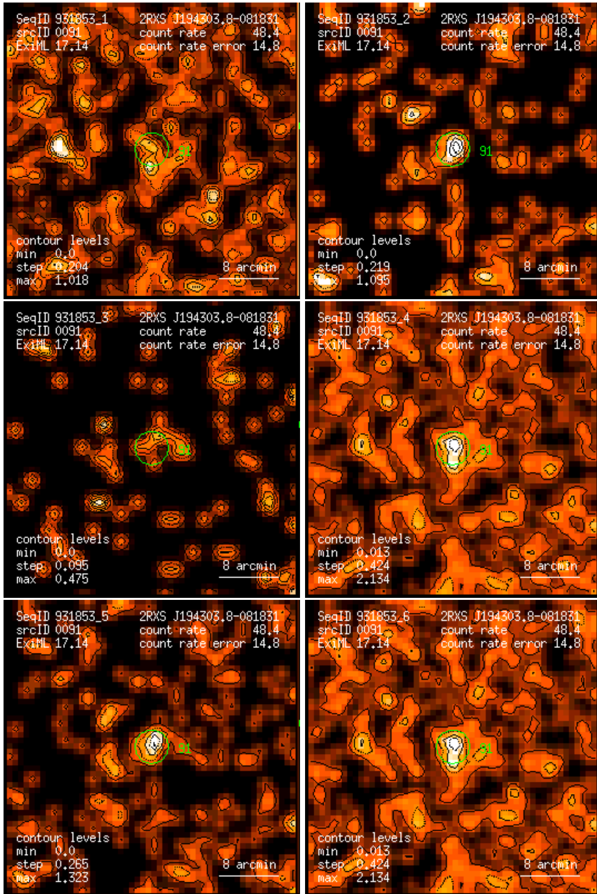
Figure 91: RASS 931853: detection 0091: band rate images, Gaussian filter: (1) PSPC channels 11 – 41, (2) 52 – 90, (3) 91 – 201, (4) 11 – 235, (5) 52 – 201, (6) 11 – 201. Broad band rates in counts/ks. Band rate contour levels in counts/ks/arcmin 2 .
