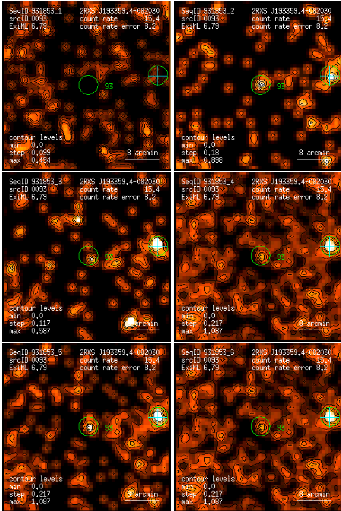
Figure 93: RASS 931853: detection 0093: band rate images, Gaussian filter: (1) PSPC channels 11 – 41, (2) 52 – 90, (3) 91 – 201, (4) 11 – 235, (5) 52 – 201, (6) 11 – 201. Broad band rates in counts/ks. Band rate contour levels in counts/ks/arcmin 2 .
