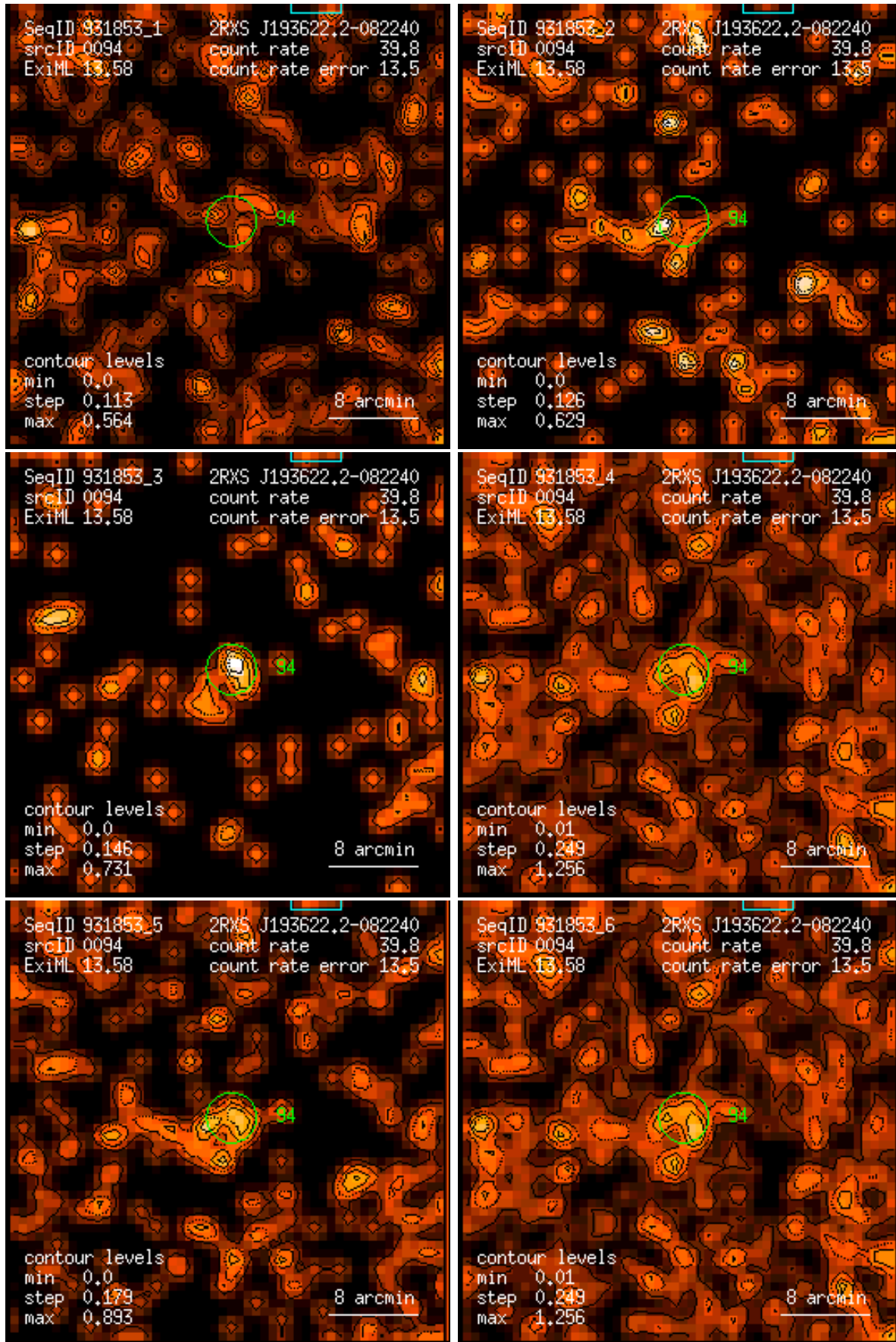
Figure 94: RASS 931853: detection 0094: band rate images, Gaussian filter: (1) PSPC channels 11 – 41, (2) 52 – 90, (3) 91 – 201, (4) 11 – 235, (5) 52 – 201, (6) 11 – 201. Broad band rates in counts/ks. Band rate contour levels in counts/ks/arcmin 2 .
