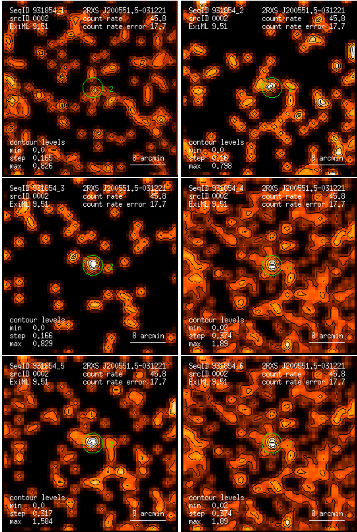
Figure 2: RASS 931854: detection 0002: band rate images, Gaussian filter: (1) PSPC channels 11 – 41, (2) 52 – 90, (3) 91 – 201, (4) 11 – 235, (5) 52 – 201, (6) 11 – 201. Broad band rates in counts/ks. Band rate contour levels in counts/ks/arcmin 2 .
