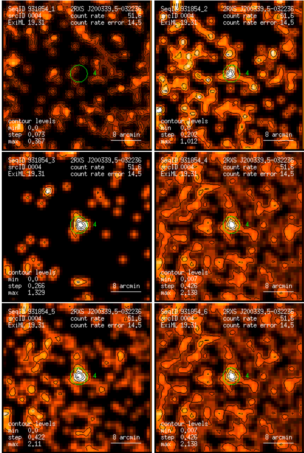
Figure 4: RASS 931854: detection 0004: band rate images, Gaussian filter: (1) PSPC channels 11 – 41, (2) 52 – 90, (3) 91 – 201, (4) 11 – 235, (5) 52 – 201, (6) 11 – 201. Broad band rates in counts/ks. Band rate contour levels in counts/ks/arcmin 2 .
