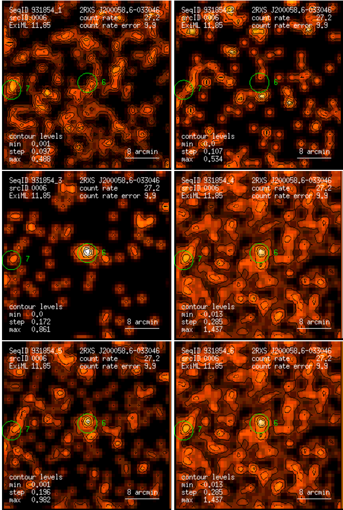
Figure 6: RASS 931854: detection 0006: band rate images, Gaussian filter: (1) PSPC channels 11 – 41, (2) 52 – 90, (3) 91 – 201, (4) 11 – 235, (5) 52 – 201, (6) 11 – 201. Broad band rates in counts/ks. Band rate contour levels in counts/ks/arcmin 2 .
