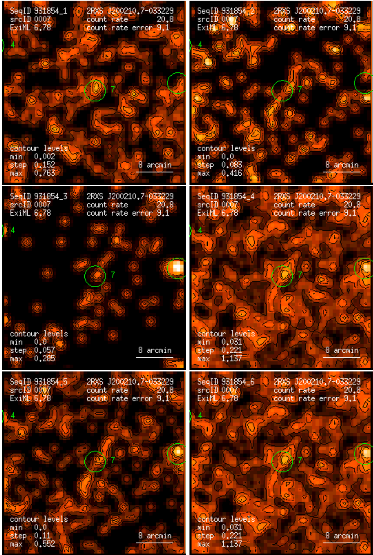
Figure 7: RASS 931854: detection 0007: band rate images, Gaussian filter: (1) PSPC channels 11 – 41, (2) 52 – 90, (3) 91 – 201, (4) 11 – 235, (5) 52 – 201, (6) 11 – 201. Broad band rates in counts/ks. Band rate contour levels in counts/ks/arcmin 2 .
