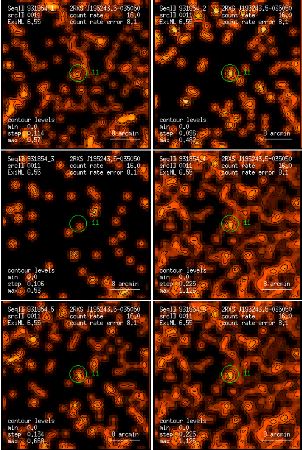
Figure 11: RASS 931854: detection 0011: band rate images, Gaussian filter: (1) PSPC channels 11 – 41, (2) 52 – 90, (3) 91 – 201, (4) 11 – 235, (5) 52 – 201, (6) 11 – 201. Broad band rates in counts/ks. Band rate contour levels in counts/ks/arcmin 2 .
