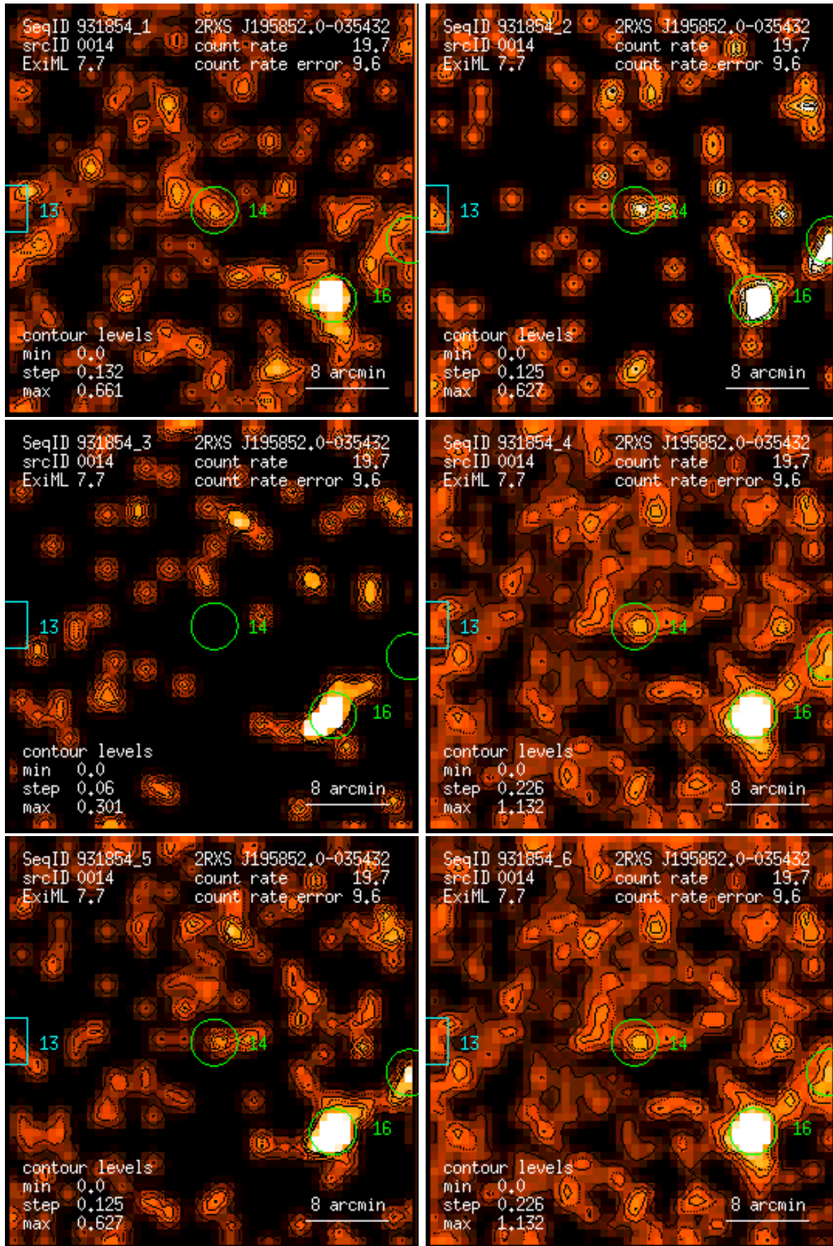
Figure 14: RASS 931854: detection 0014: band rate images, Gaussian filter: (1) PSPC channels 11 – 41, (2) 52 – 90, (3) 91 – 201, (4) 11 – 235, (5) 52 – 201, (6) 11 – 201. Broad band rates in counts/ks. Band rate contour levels in counts/ks/arcmin 2 .
