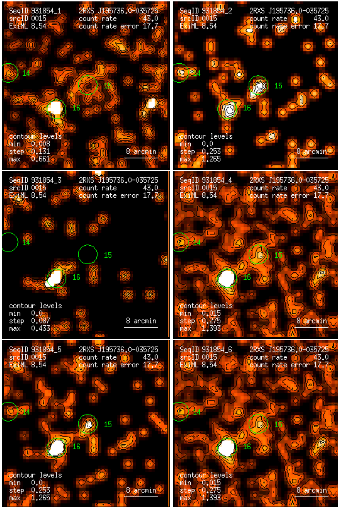
Figure 15: RASS 931854: detection 0015: band rate images, Gaussian filter: (1) PSPC channels 11 – 41, (2) 52 – 90, (3) 91 – 201, (4) 11 – 235, (5) 52 – 201, (6) 11 – 201. Broad band rates in counts/ks. Band rate contour levels in counts/ks/arcmin 2 .
