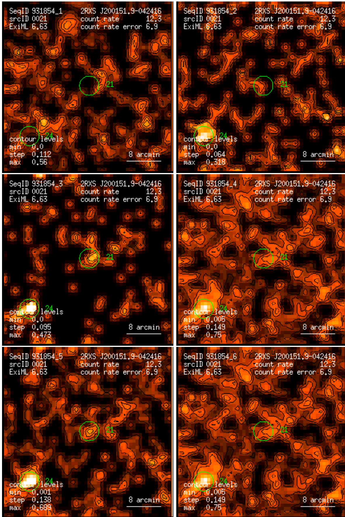
Figure 21: RASS 931854: detection 0021: band rate images, Gaussian filter: (1) PSPC channels 11 – 41, (2) 52 – 90, (3) 91 – 201, (4) 11 – 235, (5) 52 – 201, (6) 11 – 201. Broad band rates in counts/ks. Band rate contour levels in counts/ks/arcmin 2 .
