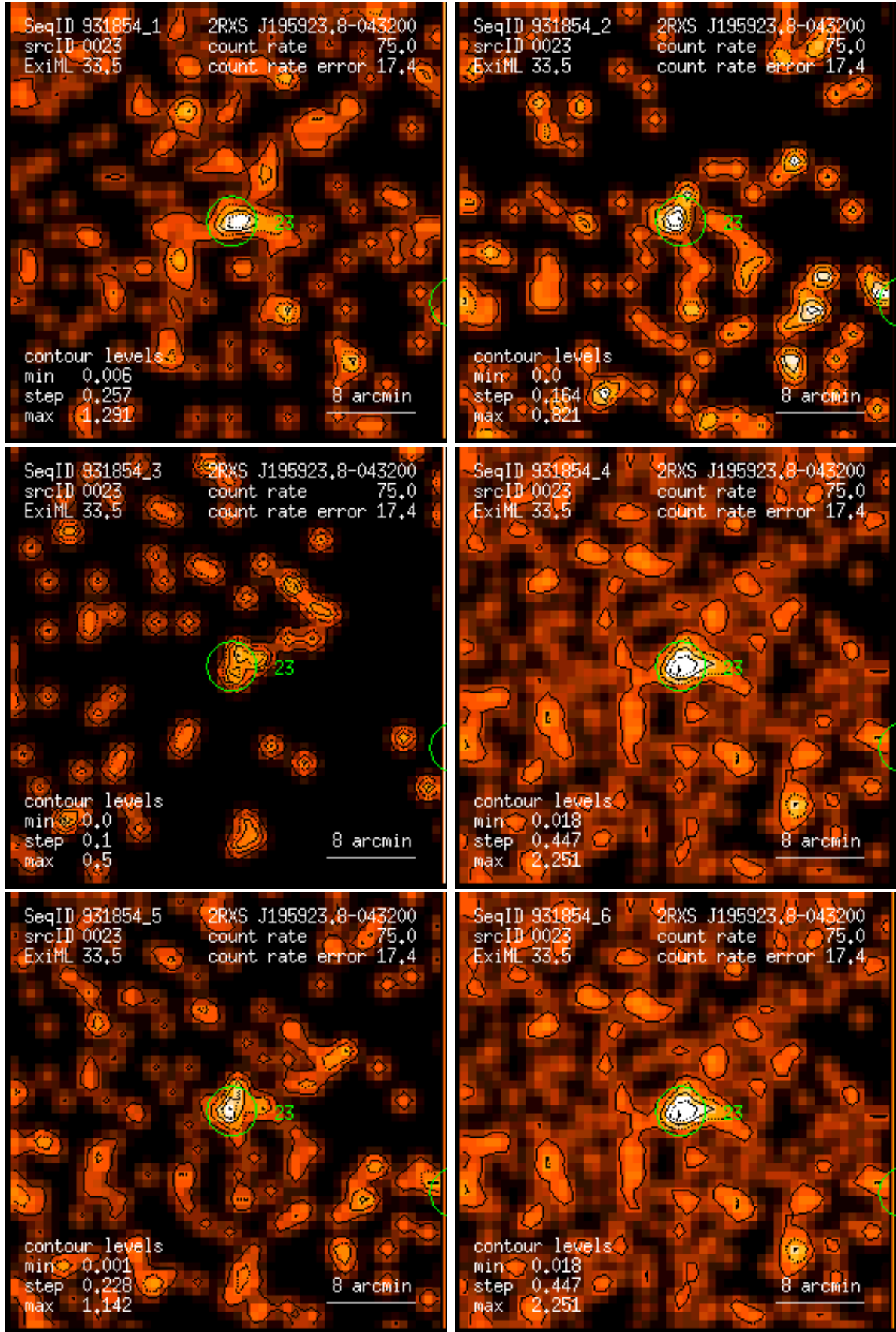
Figure 23: RASS 931854: detection 0023: band rate images, Gaussian filter: (1) PSPC channels 11 – 41, (2) 52 – 90, (3) 91 – 201, (4) 11 – 235, (5) 52 – 201, (6) 11 – 201. Broad band rates in counts/ks. Band rate contour levels in counts/ks/arcmin 2 .
