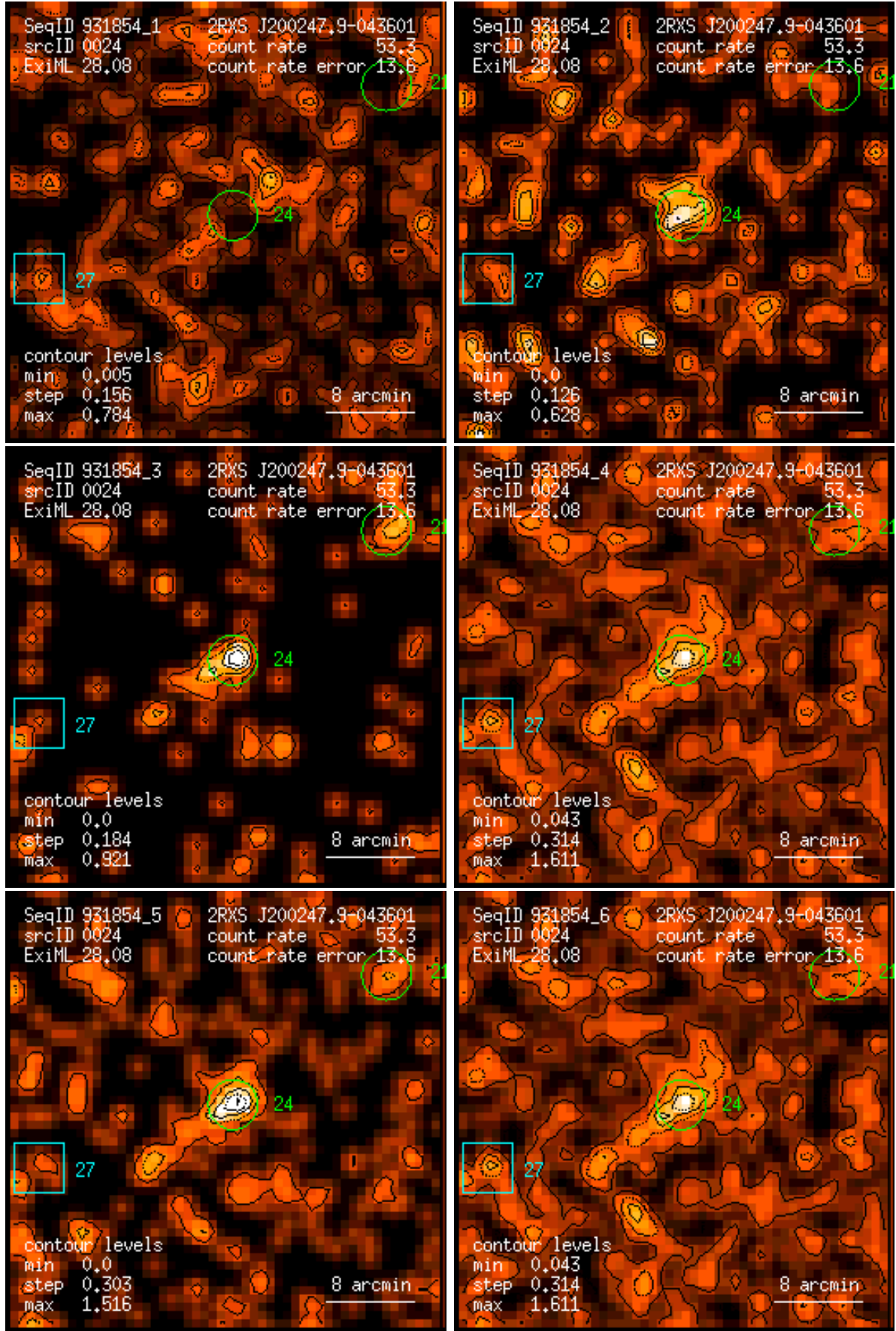
Figure 24: RASS 931854: detection 0024: band rate images, Gaussian filter: (1) PSPC channels 11 – 41, (2) 52 – 90, (3) 91 – 201, (4) 11 – 235, (5) 52 – 201, (6) 11 – 201. Broad band rates in counts/ks. Band rate contour levels in counts/ks/arcmin 2 .
