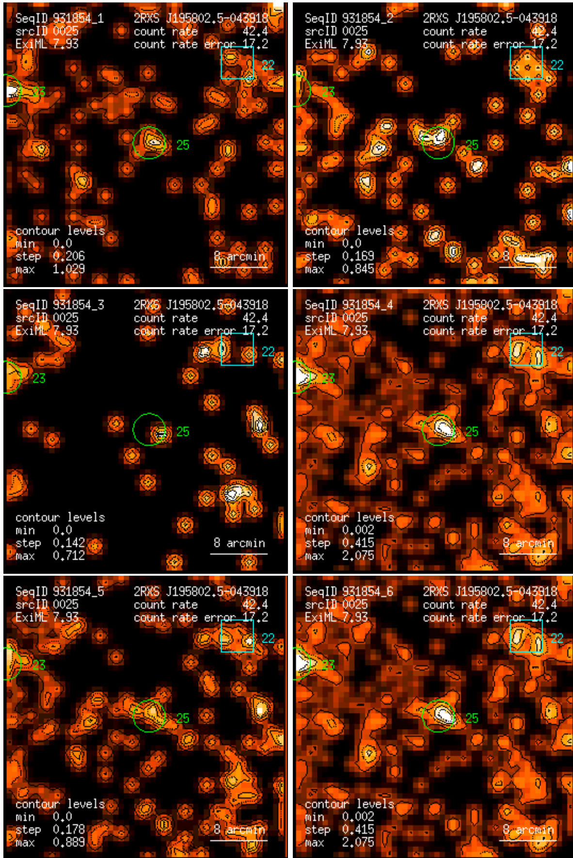
Figure 25: RASS 931854: detection 0025: band rate images, Gaussian filter: (1) PSPC channels 11 – 41, (2) 52 – 90, (3) 91 – 201, (4) 11 – 235, (5) 52 – 201, (6) 11 – 201. Broad band rates in counts/ks. Band rate contour levels in counts/ks/arcmin 2 .
