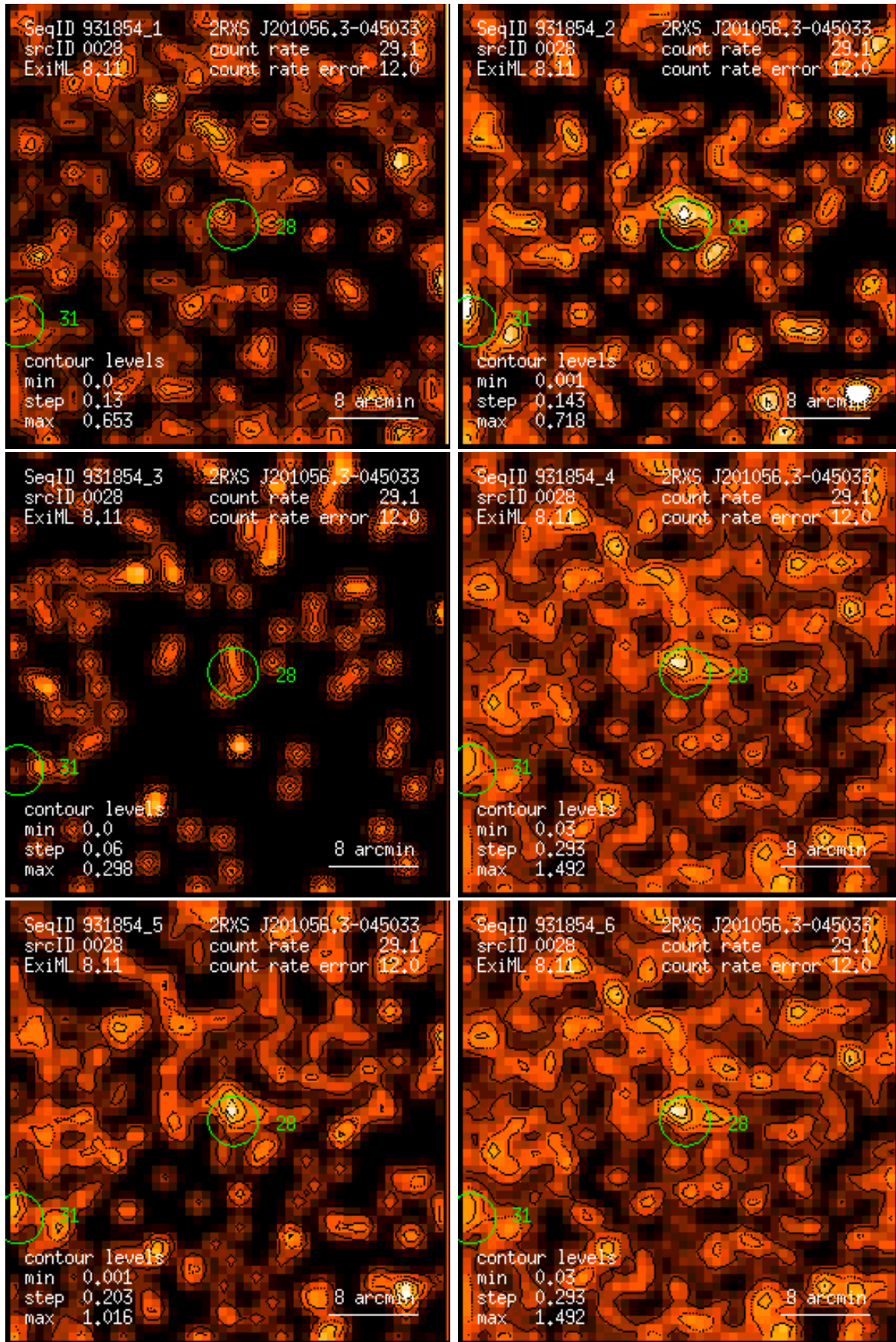
Figure 28: RASS 931854: detection 0028: band rate images, Gaussian filter: (1) PSPC channels 11 – 41, (2) 52 – 90, (3) 91 – 201, (4) 11 – 235, (5) 52 – 201, (6) 11 – 201. Broad band rates in counts/ks. Band rate contour levels in counts/ks/arcmin 2 .
