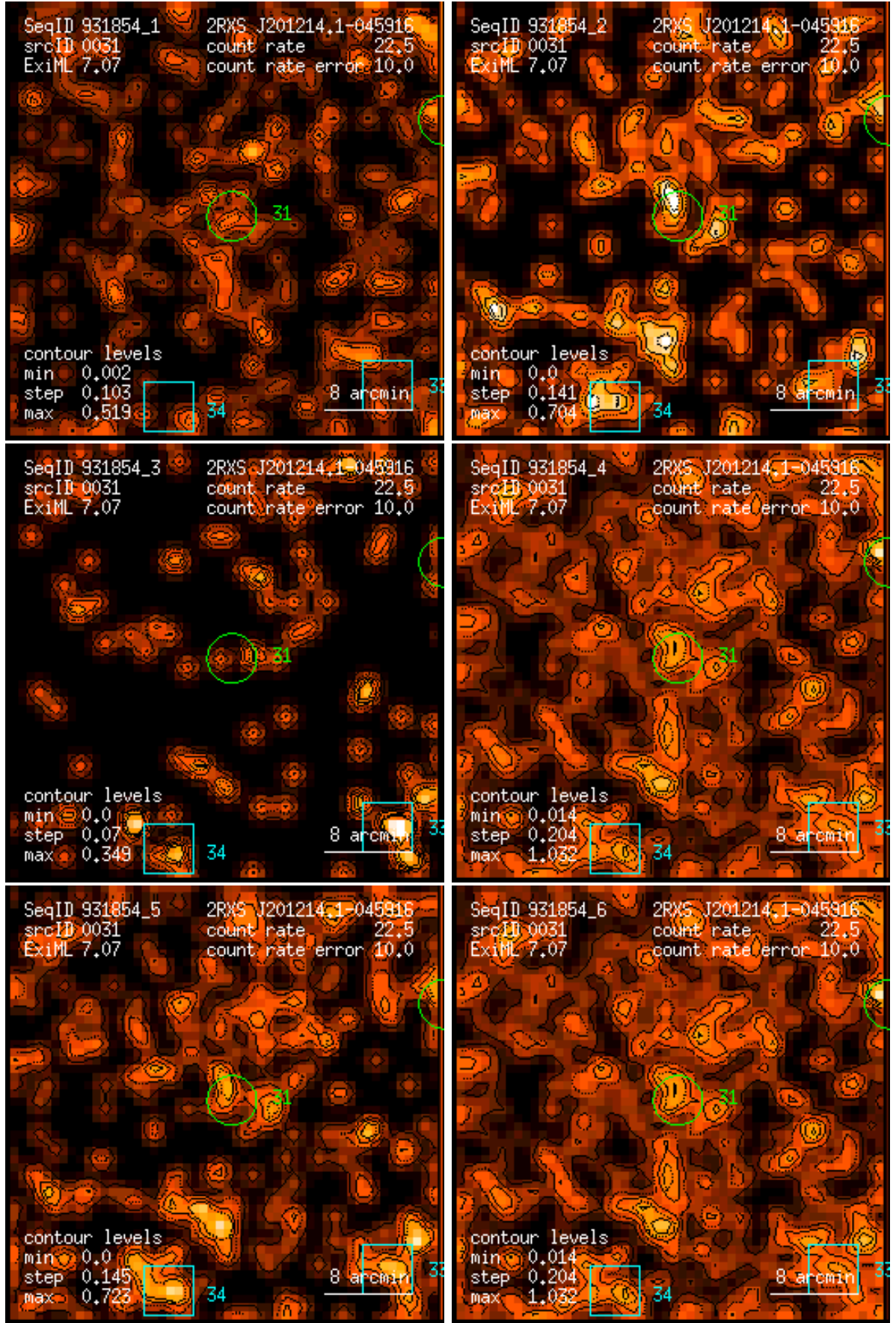
Figure 31: RASS 931854: detection 0031: band rate images, Gaussian filter: (1) PSPC channels 11 – 41, (2) 52 – 90, (3) 91 – 201, (4) 11 – 235, (5) 52 – 201, (6) 11 – 201. Broad band rates in counts/ks. Band rate contour levels in counts/ks/arcmin 2 .
