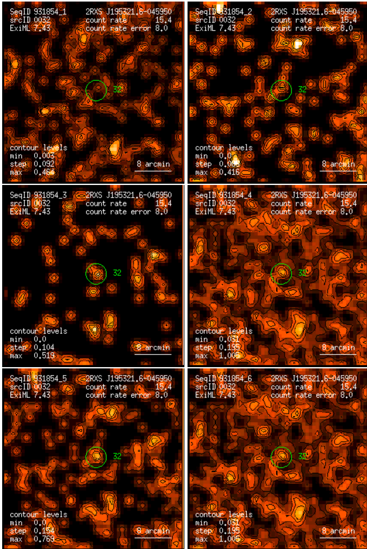
Figure 32: RASS 931854: detection 0032: band rate images, Gaussian filter: (1) PSPC channels 11 – 41, (2) 52 – 90, (3) 91 – 201, (4) 11 – 235, (5) 52 – 201, (6) 11 – 201. Broad band rates in counts/ks. Band rate contour levels in counts/ks/arcmin 2 .
