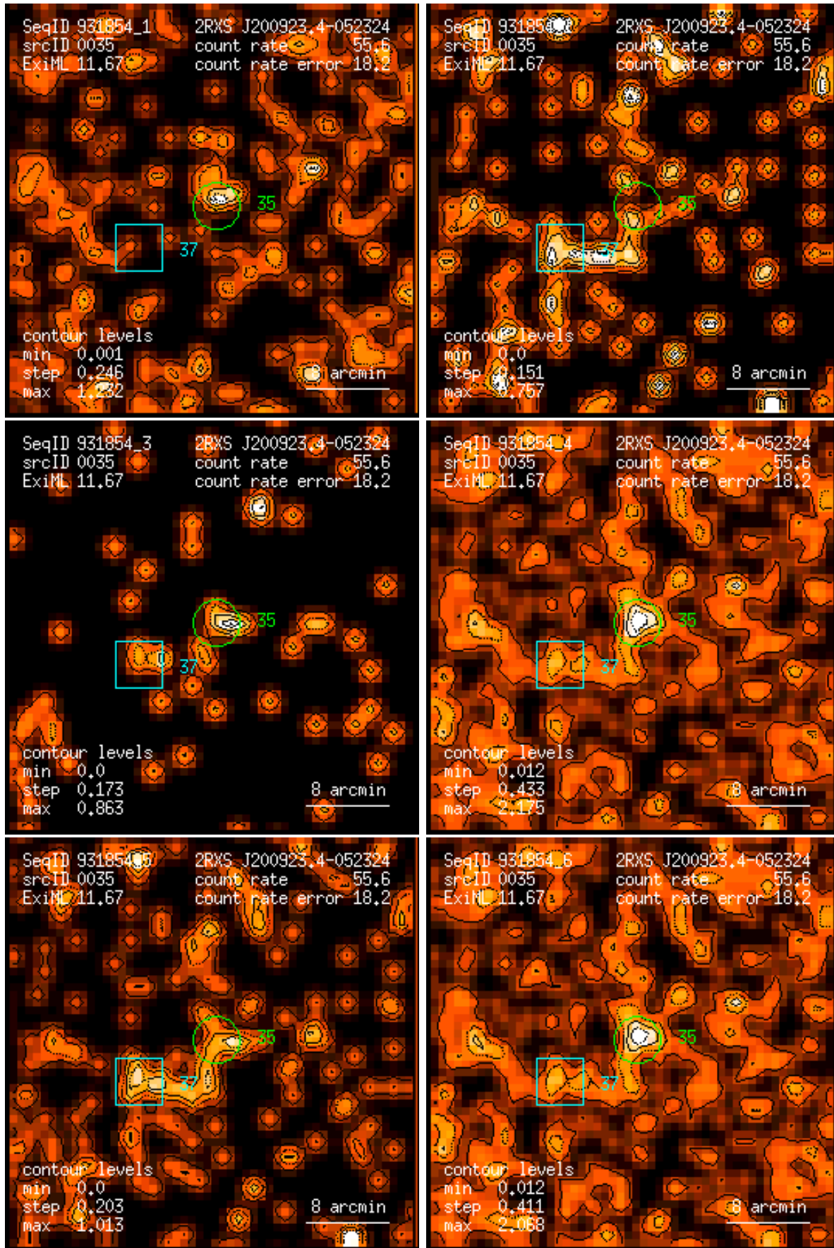
Figure 35: RASS 931854: detection 0035: band rate images, Gaussian filter: (1) PSPC channels 11 – 41, (2) 52 – 90, (3) 91 – 201, (4) 11 – 235, (5) 52 – 201, (6) 11 – 201. Broad band rates in counts/ks. Band rate contour levels in counts/ks/arcmin 2 .
