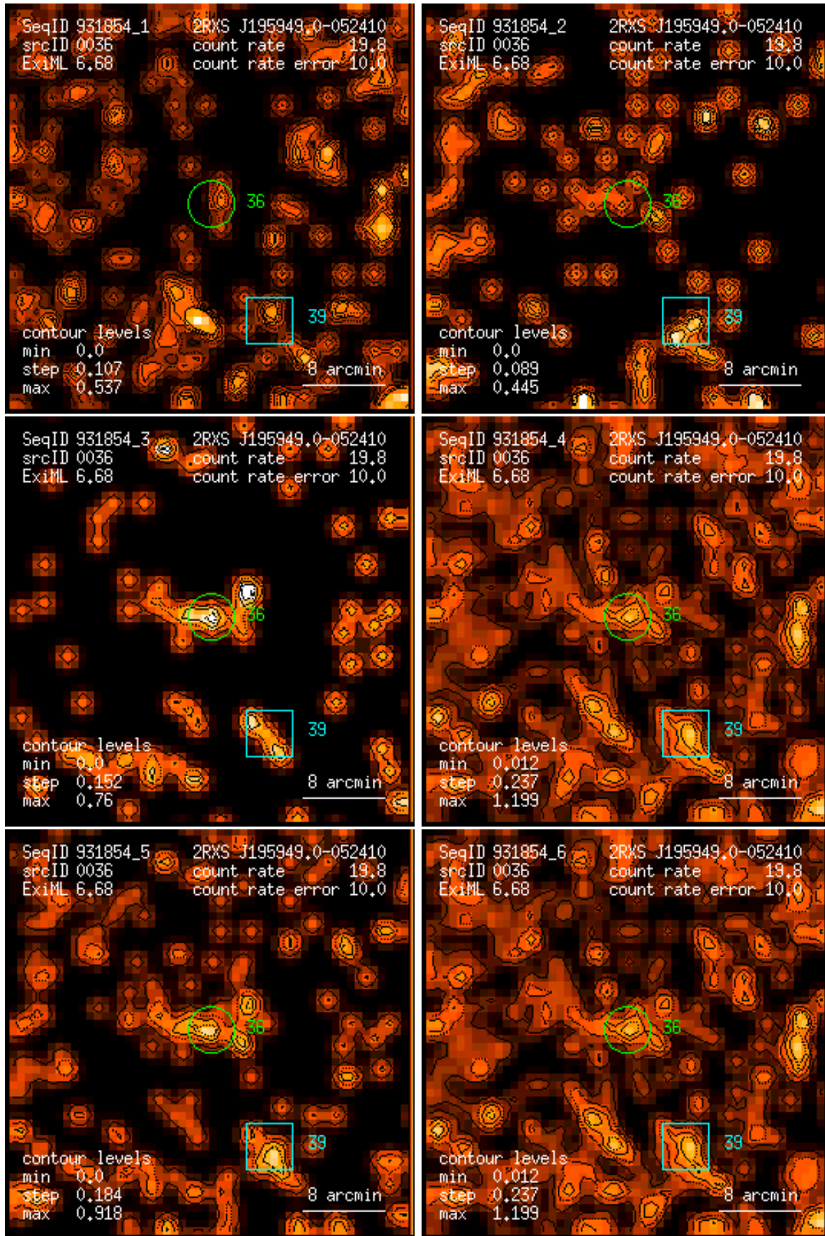
Figure 36: RASS 931854: detection 0036: band rate images, Gaussian filter: (1) PSPC channels 11 – 41, (2) 52 – 90, (3) 91 – 201, (4) 11 – 235, (5) 52 – 201, (6) 11 – 201. Broad band rates in counts/ks. Band rate contour levels in counts/ks/arcmin 2 .
