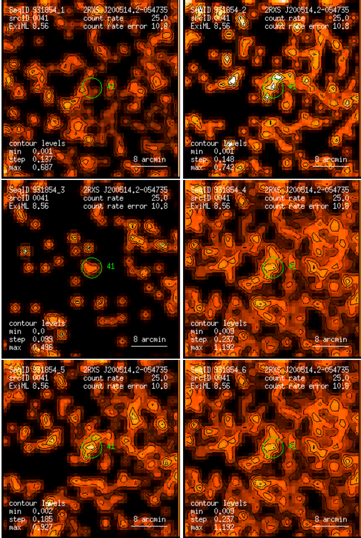
Figure 41: RASS 931854: detection 0041: band rate images, Gaussian filter: (1) PSPC channels 11 – 41, (2) 52 – 90, (3) 91 – 201, (4) 11 – 235, (5) 52 – 201, (6) 11 – 201. Broad band rates in counts/ks. Band rate contour levels in counts/ks/arcmin 2 .
