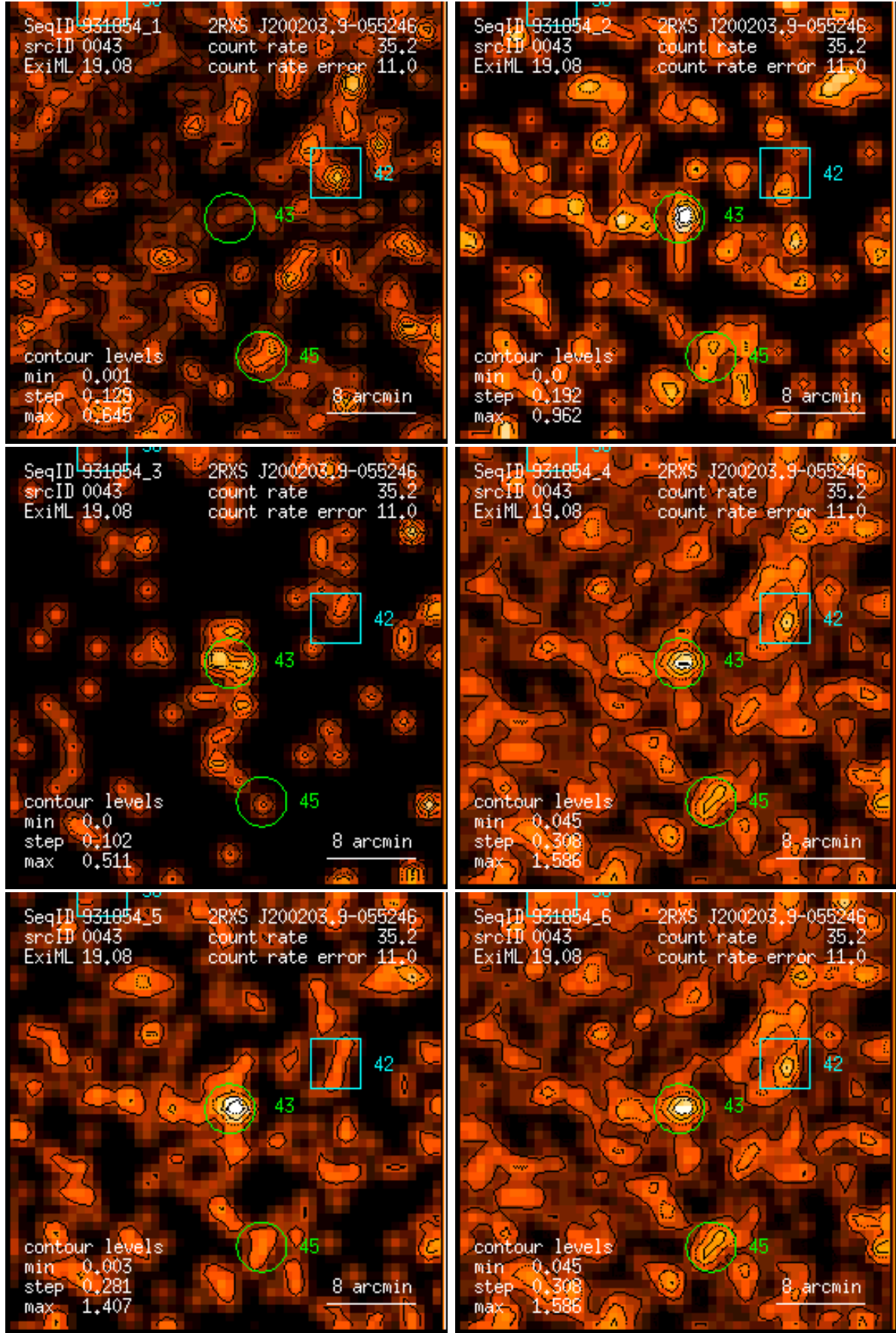
Figure 43: RASS 931854: detection 0043: band rate images, Gaussian filter: (1) PSPC channels 11 – 41, (2) 52 – 90, (3) 91 – 201, (4) 11 – 235, (5) 52 – 201, (6) 11 – 201. Broad band rates in counts/ks. Band rate contour levels in counts/ks/arcmin 2 .
