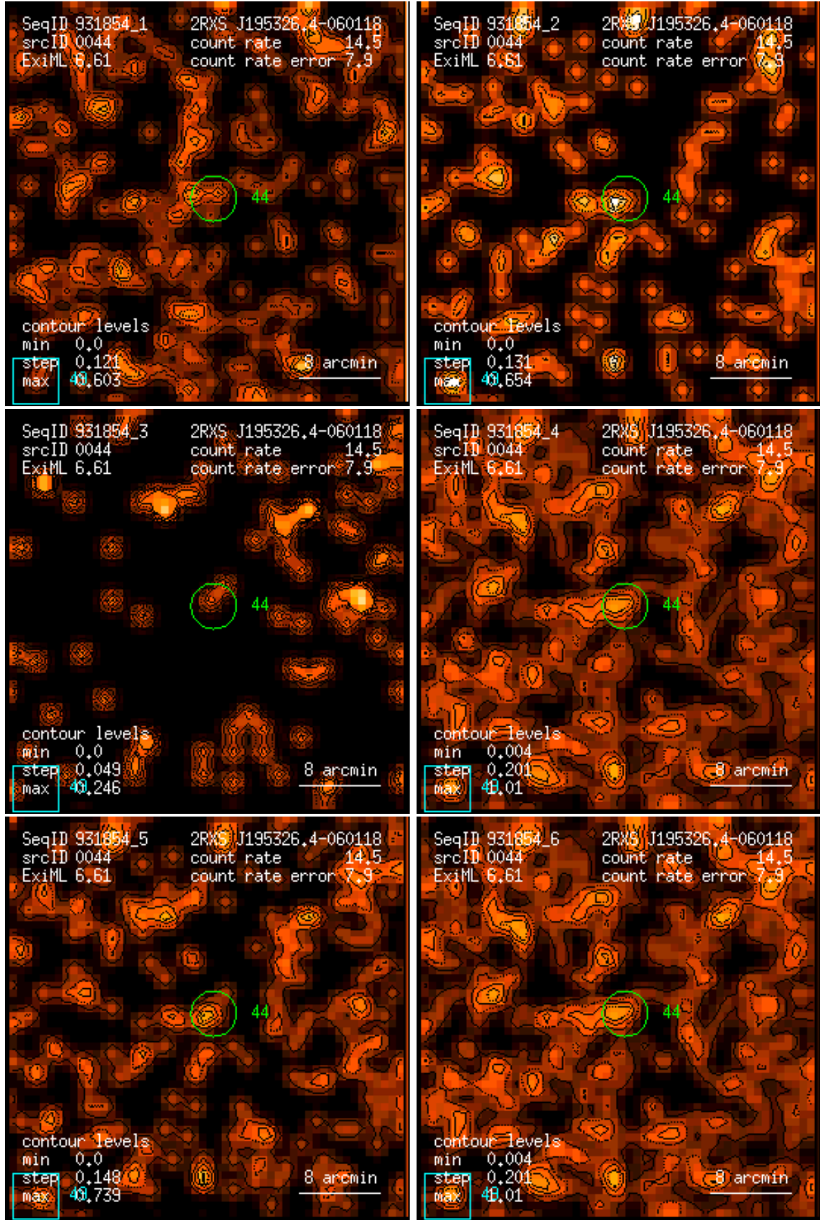
Figure 44: RASS 931854: detection 0044: band rate images, Gaussian filter: (1) PSPC channels 11 – 41, (2) 52 – 90, (3) 91 – 201, (4) 11 – 235, (5) 52 – 201, (6) 11 – 201. Broad band rates in counts/ks. Band rate contour levels in counts/ks/arcmin 2 .
