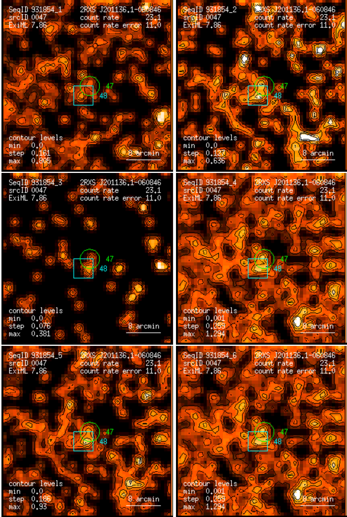
Figure 47: RASS 931854: detection 0047: band rate images, Gaussian filter: (1) PSPC channels 11 – 41, (2) 52 – 90, (3) 91 – 201, (4) 11 – 235, (5) 52 – 201, (6) 11 – 201. Broad band rates in counts/ks. Band rate contour levels in counts/ks/arcmin 2 .
