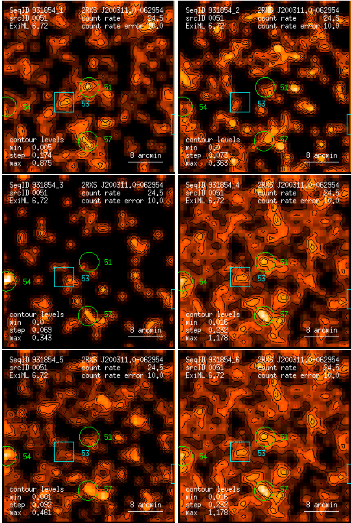
Figure 51: RASS 931854: detection 0051: band rate images, Gaussian filter: (1) PSPC channels 11 – 41, (2) 52 – 90, (3) 91 – 201, (4) 11 – 235, (5) 52 – 201, (6) 11 – 201. Broad band rates in counts/ks. Band rate contour levels in counts/ks/arcmin 2 .
