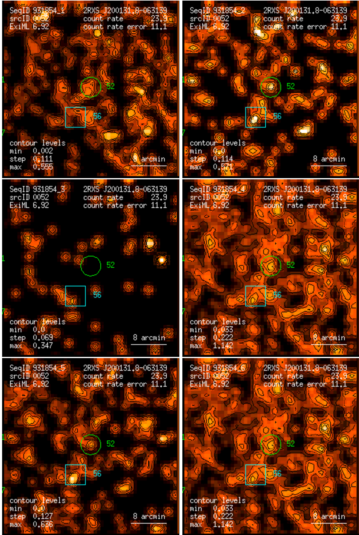
Figure 52: RASS 931854: detection 0052: band rate images, Gaussian filter: (1) PSPC channels 11 – 41, (2) 52 – 90, (3) 91 – 201, (4) 11 – 235, (5) 52 – 201, (6) 11 – 201. Broad band rates in counts/ks. Band rate contour levels in counts/ks/arcmin 2 .
