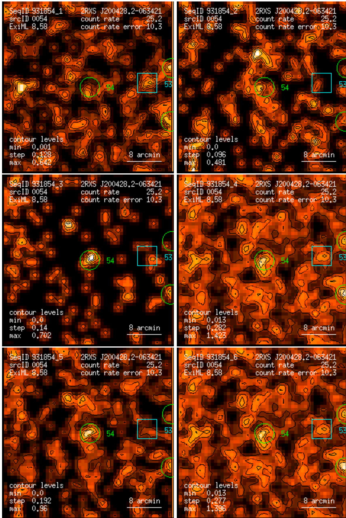
Figure 54: RASS 931854: detection 0054: band rate images, Gaussian filter: (1) PSPC channels 11 – 41, (2) 52 – 90, (3) 91 – 201, (4) 11 – 235, (5) 52 – 201, (6) 11 – 201. Broad band rates in counts/ks. Band rate contour levels in counts/ks/arcmin 2 .
