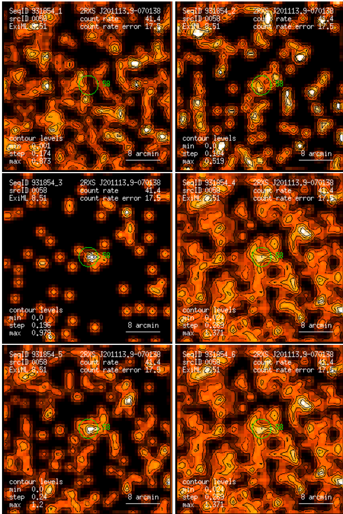
Figure 58: RASS 931854: detection 0058: band rate images, Gaussian filter: (1) PSPC channels 11 – 41, (2) 52 – 90, (3) 91 – 201, (4) 11 – 235, (5) 52 – 201, (6) 11 – 201. Broad band rates in counts/ks. Band rate contour levels in counts/ks/arcmin 2 .
