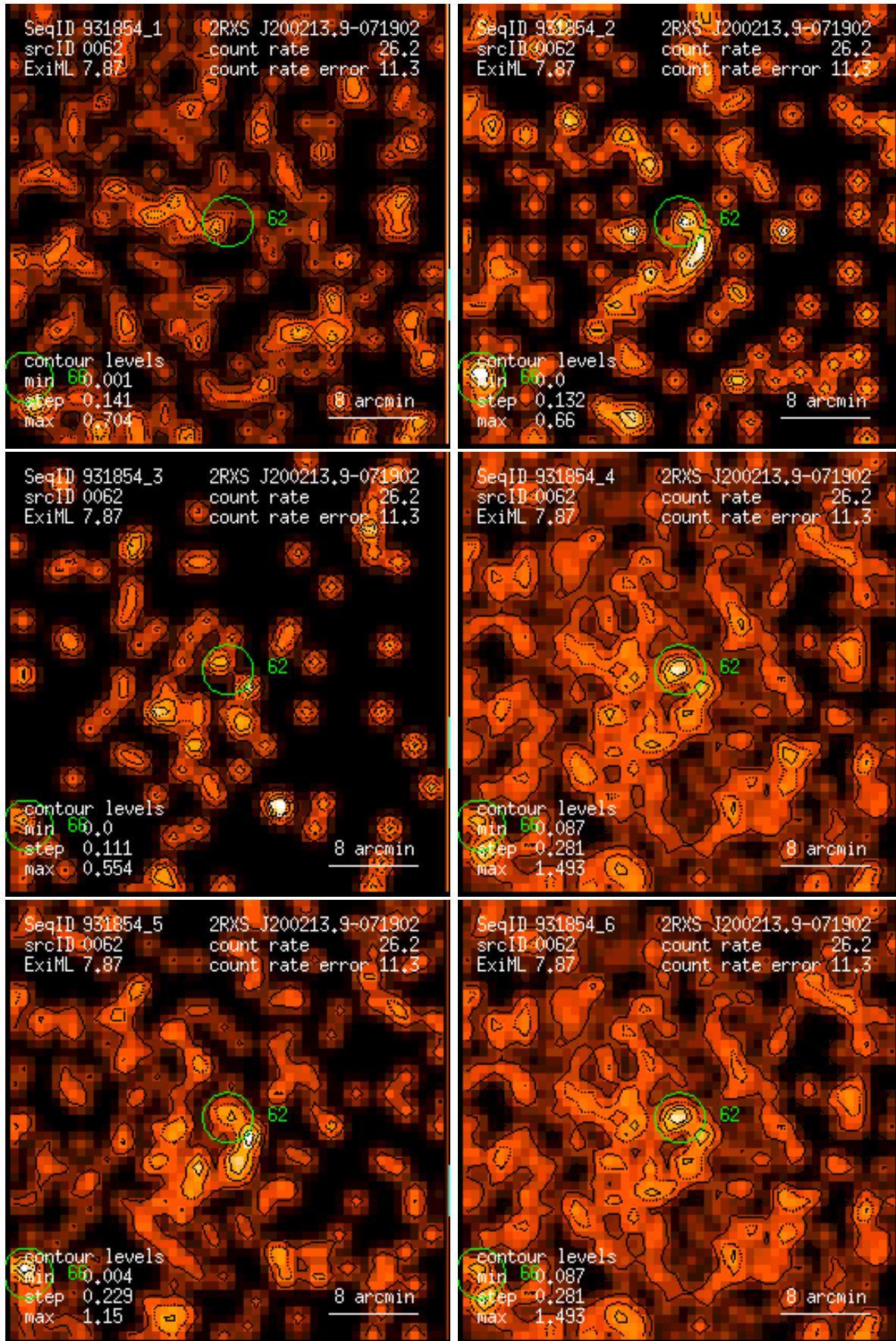
Figure 62: RASS 931854: detection 0062: band rate images, Gaussian filter: (1) PSPC channels 11 – 41, (2) 52 – 90, (3) 91 – 201, (4) 11 – 235, (5) 52 – 201, (6) 11 – 201. Broad band rates in counts/ks. Band rate contour levels in counts/ks/arcmin 2 .
