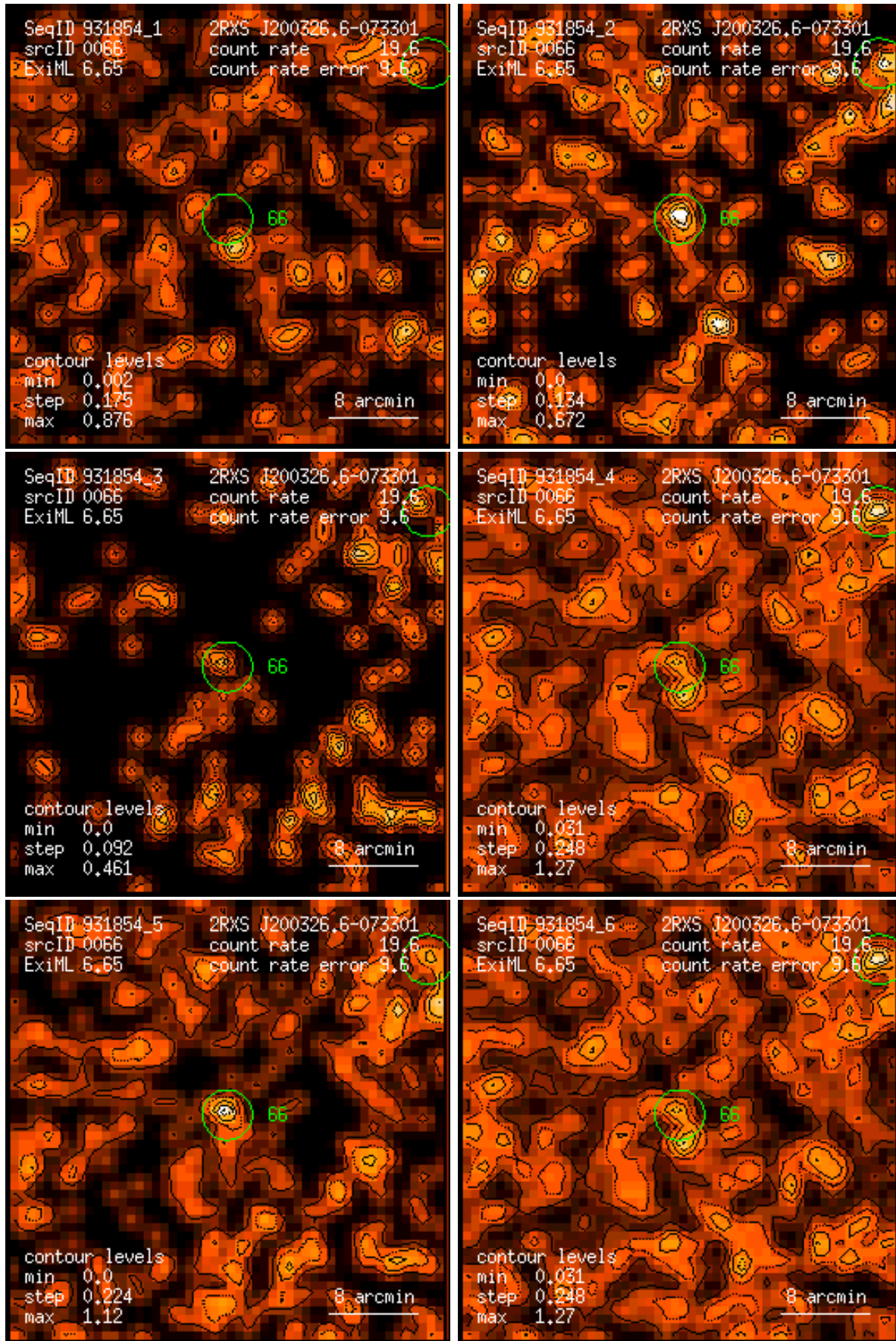
Figure 66: RASS 931854: detection 0066: band rate images, Gaussian filter: (1) PSPC channels 11 – 41, (2) 52 – 90, (3) 91 – 201, (4) 11 – 235, (5) 52 – 201, (6) 11 – 201. Broad band rates in counts/ks. Band rate contour levels in counts/ks/arcmin 2 .
