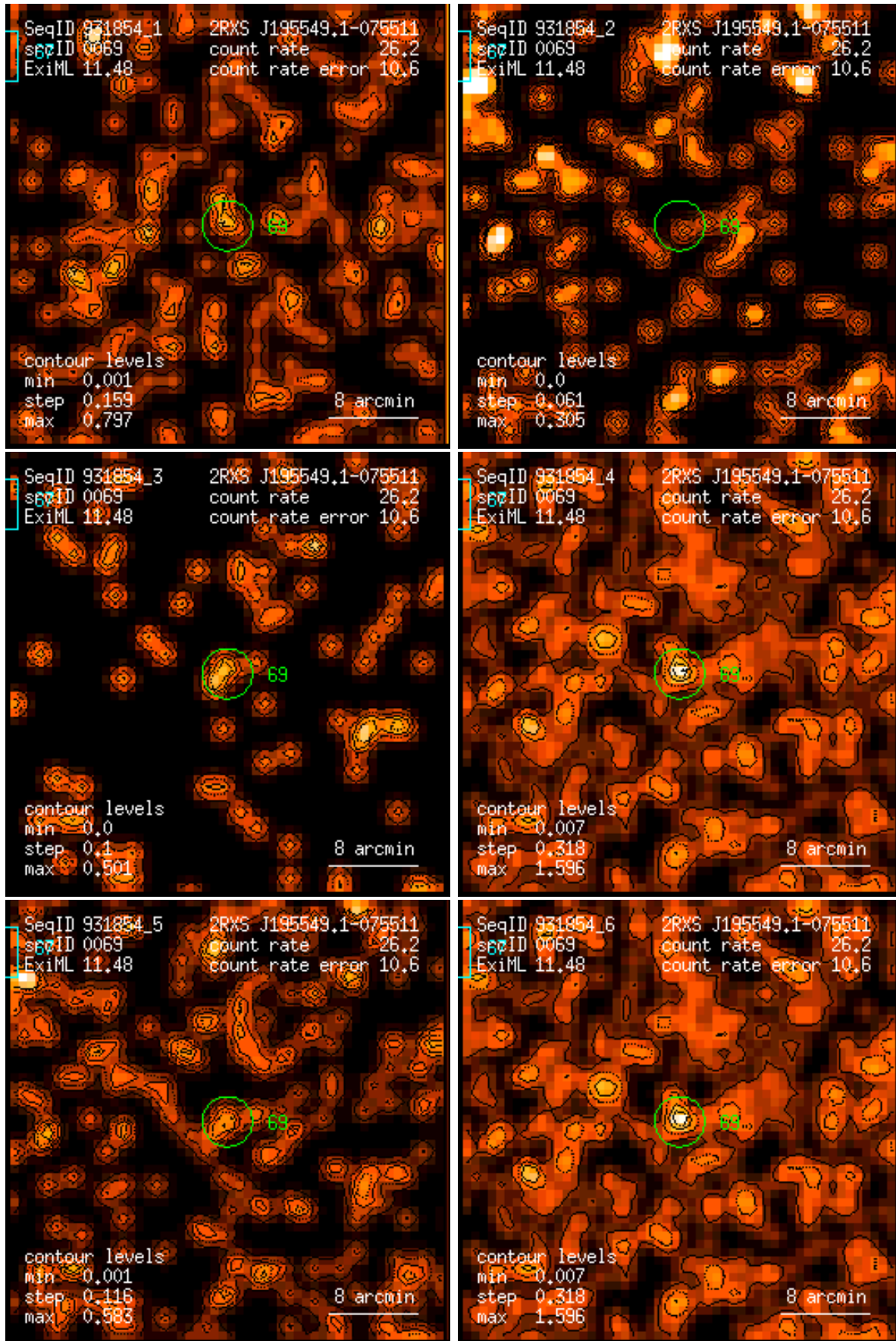
Figure 69: RASS 931854: detection 0069: band rate images, Gaussian filter: (1) PSPC channels 11 – 41, (2) 52 – 90, (3) 91 – 201, (4) 11 – 235, (5) 52 – 201, (6) 11 – 201. Broad band rates in counts/ks. Band rate contour levels in counts/ks/arcmin 2 .
