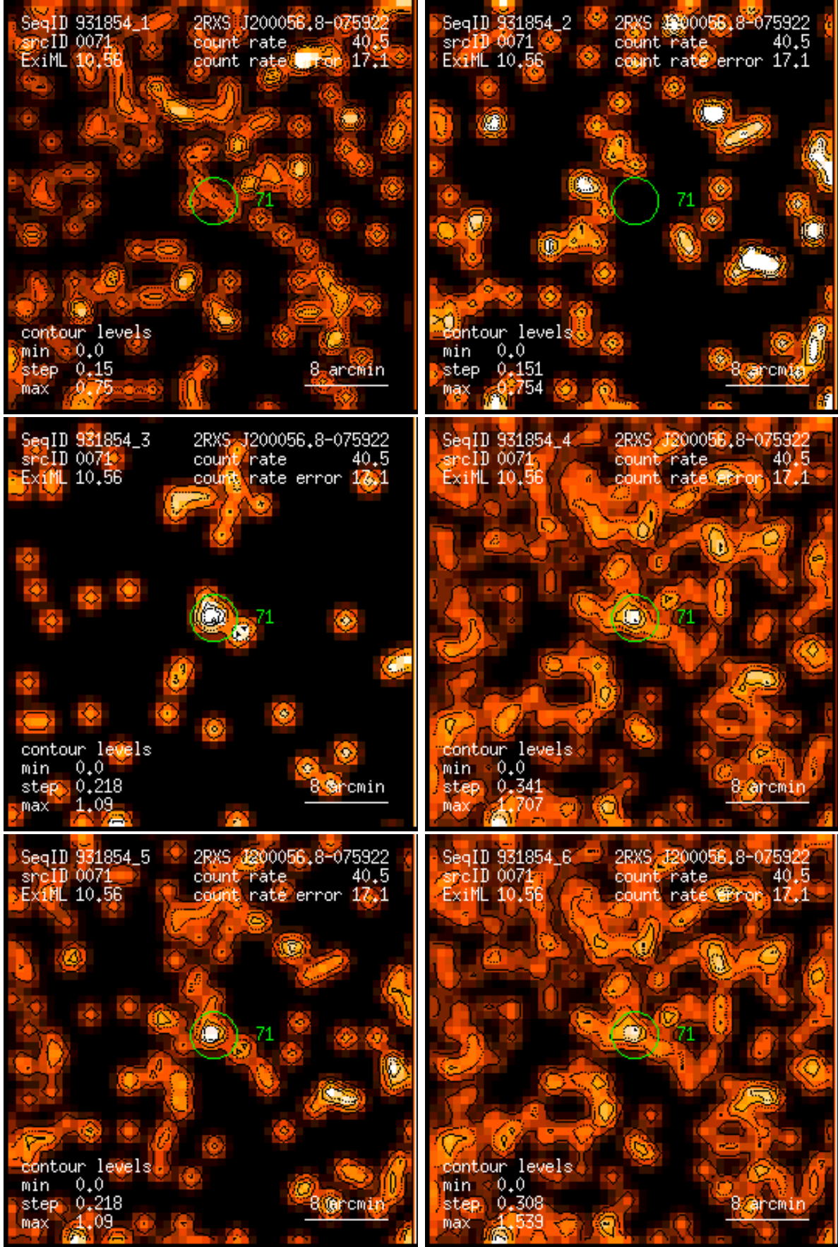
Figure 71: RASS 931854: detection 0071: band rate images, Gaussian filter: (1) PSPC channels 11 – 41, (2) 52 – 90, (3) 91 – 201, (4) 11 – 235, (5) 52 – 201, (6) 11 – 201. Broad band rates in counts/ks. Band rate contour levels in counts/ks/arcmin 2 .
